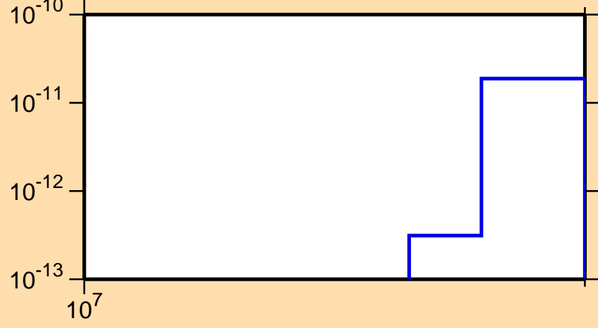
\sigma vs. E for ^{175}\text{Hf} (mt 45)
