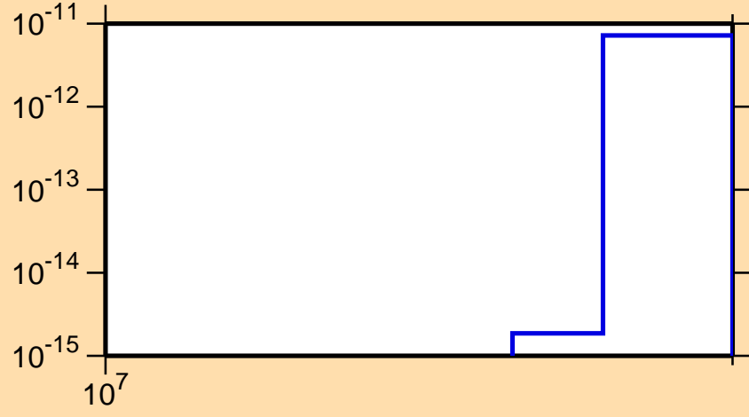
\sigma vs. E for ^{175}\text{Hf} (mt 34)
