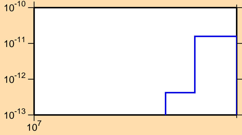
\sigma vs. E for ^{175}\text{Hf}(\text{mt117})
