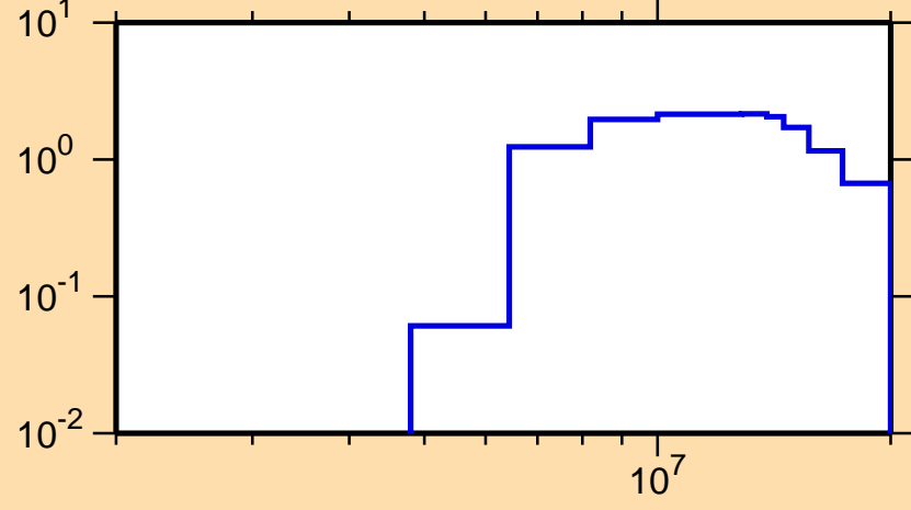
\sigma vs. E for ^{185}\text{W}(n,2n)
