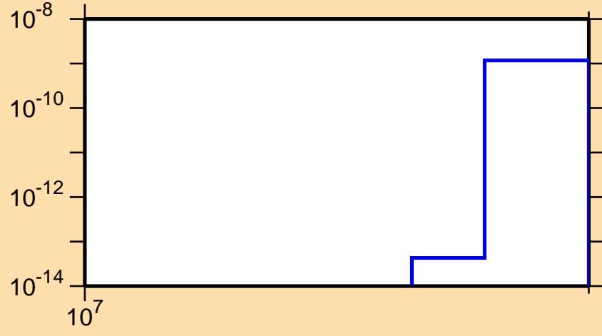
\sigma vs. E for ^{179}\text{Ta}(n,3n\alpha)
