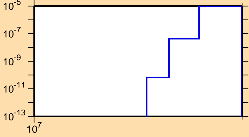
\sigma vs. E for ^{179}\text{Ta}(n,2np)
