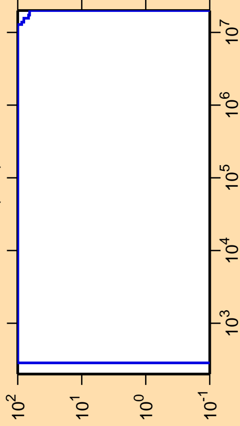
\Delta\sigma/\sigma vs. E for ^{179}\text{Ta}(n,\alpha)
