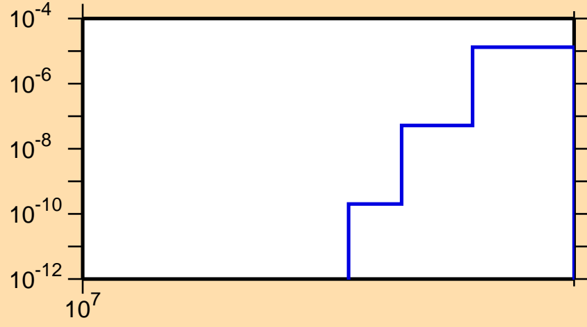
\sigma vs. E for ^{179}\text{Ta}(n,nt)
