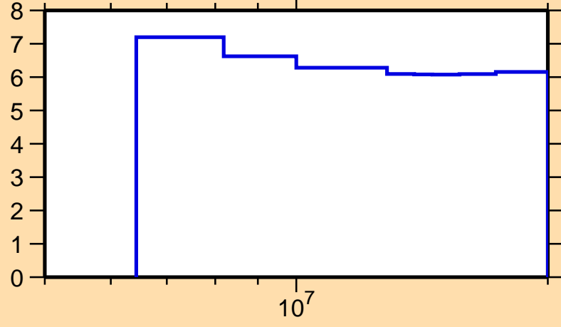
\Delta\sigma/\sigma vs. E for ^{179}\text{Ta}(n,\text{nonel.})
