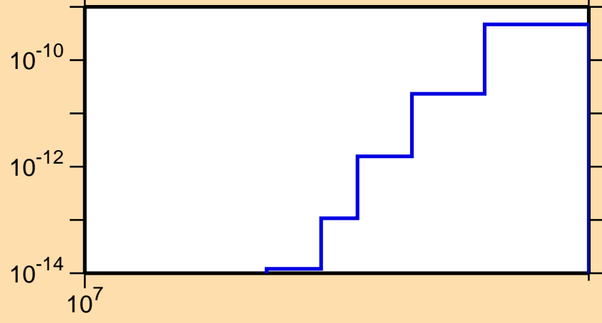
\sigma vs. E for ^{179}\text{Ta}(\text{mt117})
