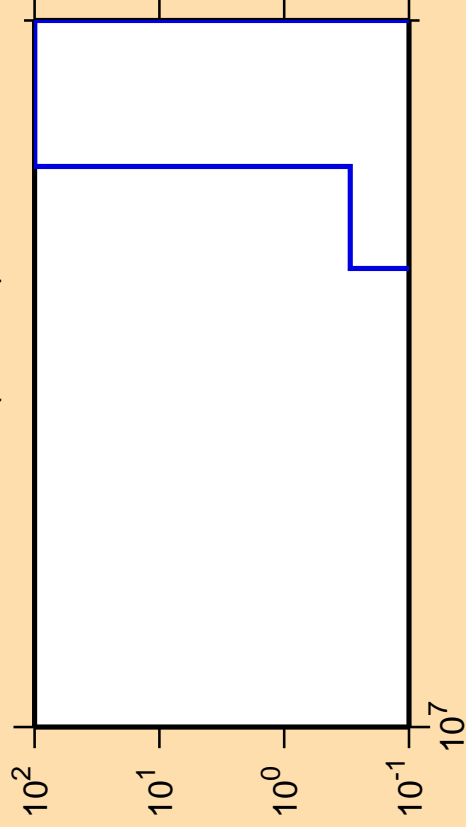
\Delta\sigma/\sigma vs. E for ^{181}\text{Hf}(n,\text{He3})
