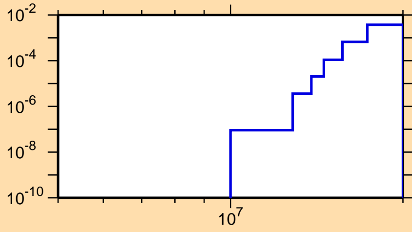
\sigma vs. E for ^{181}\text{Hf}(n,np)
