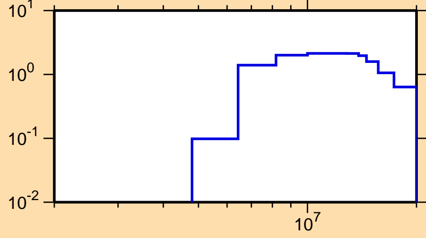
\sigma vs. E for ^{181}\text{Hf}(n,2n)
