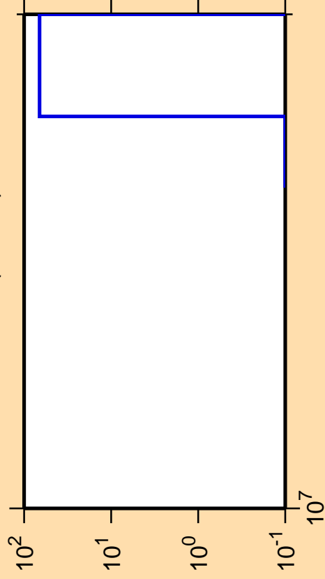
\Delta\sigma/\sigma vs. E for ^{175}\text{Lu}(n,3n\alpha)
