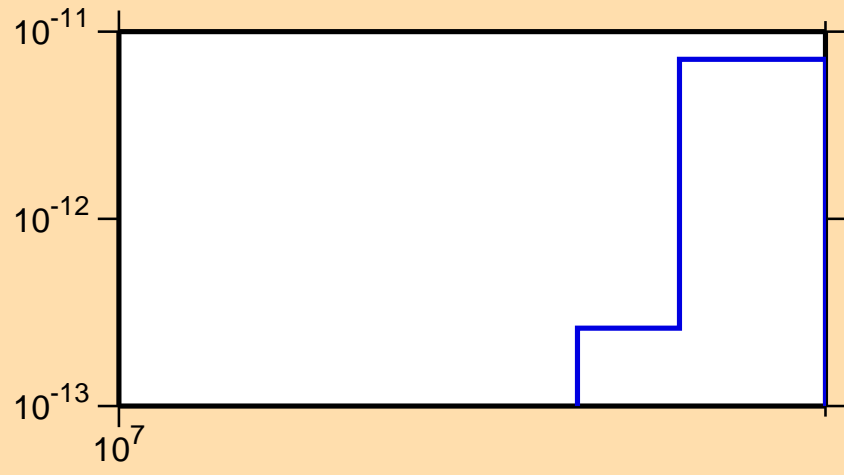
\sigma vs. E for ^{175}\text{Lu}(\text{mt117})
