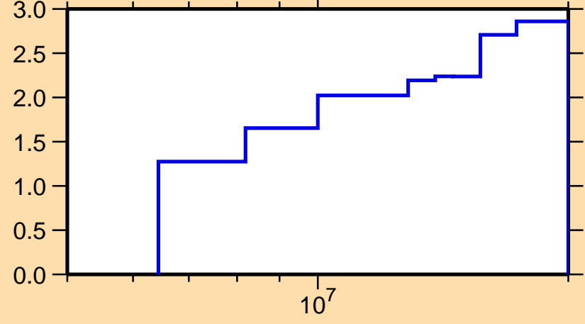
\Delta\sigma/\sigma vs. E for ^{175}\text{Lu}(n,\text{el.})
