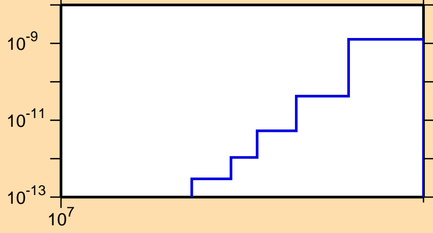
\sigma vs. E for ^{175}\text{Lu}(n,p\alpha)
