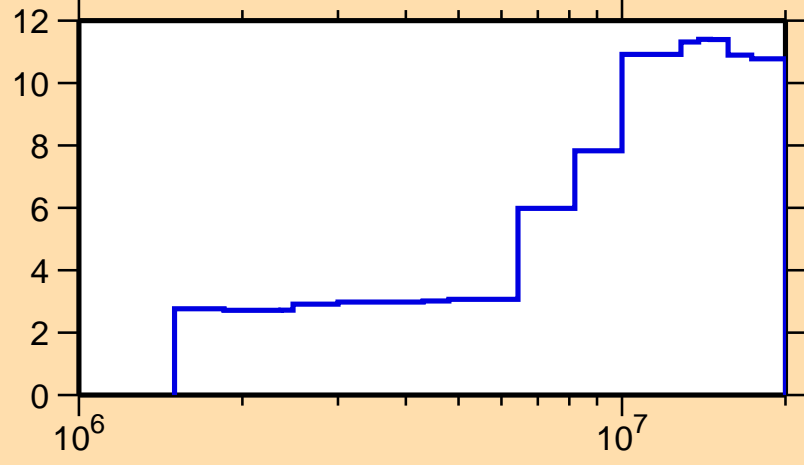
\Delta\sigma/\sigma vs. E for ^{175}\text{Lu}(n,ncont.)
