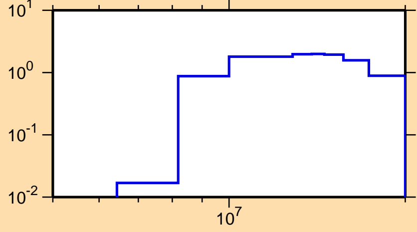
\sigma vs. E for ^{175}\text{Lu}(n,2n)
