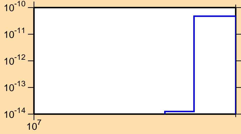
\sigma vs. E for ^{175}\text{Lu}(n,3n\alpha)
