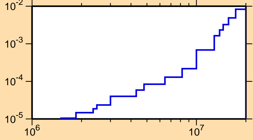
\sigma vs. E for ^{174}\text{Hf}(n,\alpha)
