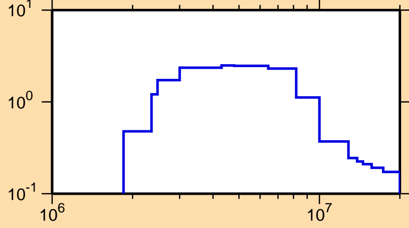
\sigma vs. E for ^{174}\text{Yb}(n,n\text{cont.})
