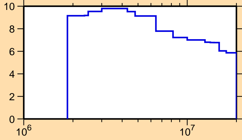
\Delta\sigma/\sigma vs. E for ^{174}\text{Yb}(n,n\text{onel.})
