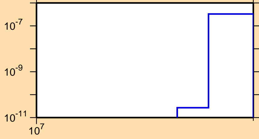
\sigma vs. E for ^{174}\text{Yb}(n,2np)
