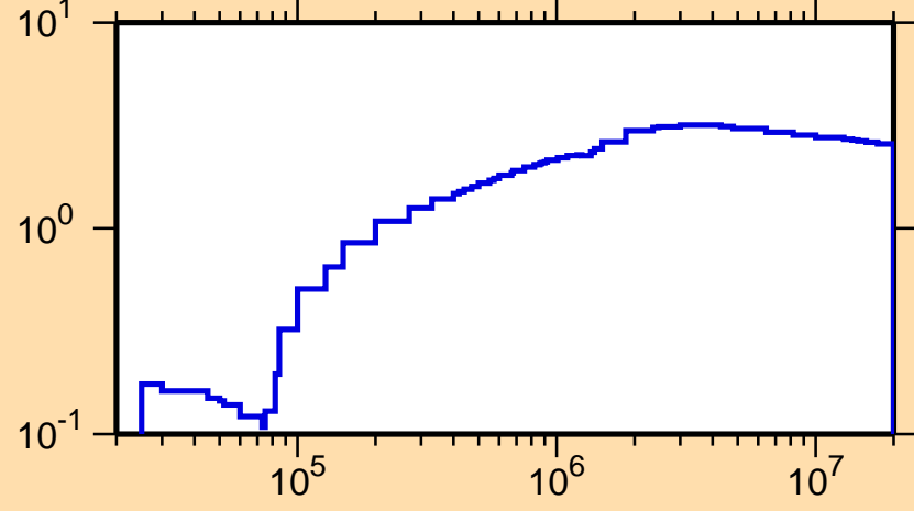
\sigma vs. E for ^{174}\text{Yb}(n,\text{nonel.})
