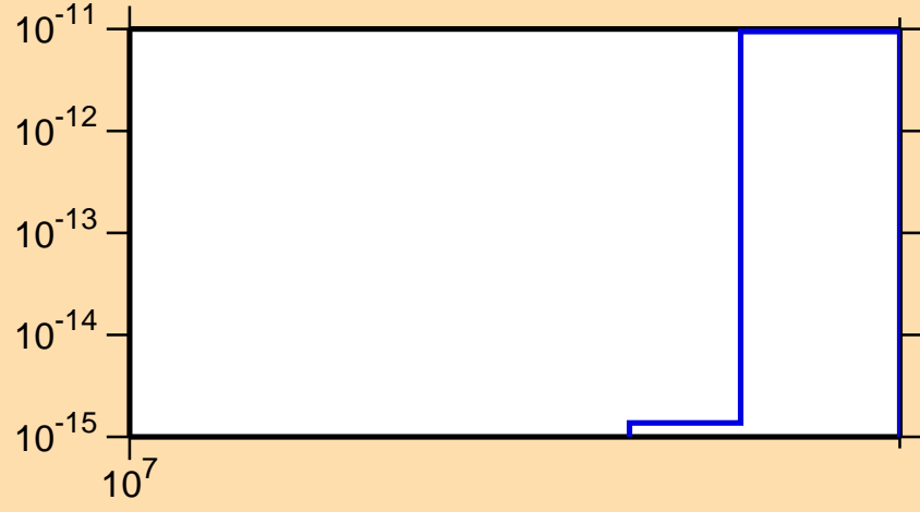
\sigma vs. E for ^{170}\text{Er}(n,3n\alpha)
