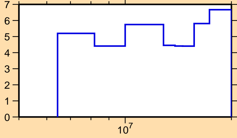
\Delta\sigma/\sigma vs. E for ^{170}\text{Er}(n,\text{el.})
