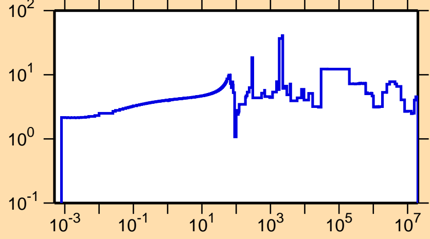
\Delta\sigma/\sigma vs. E for ^{170}\text{Er}(n,\text{tot.})
