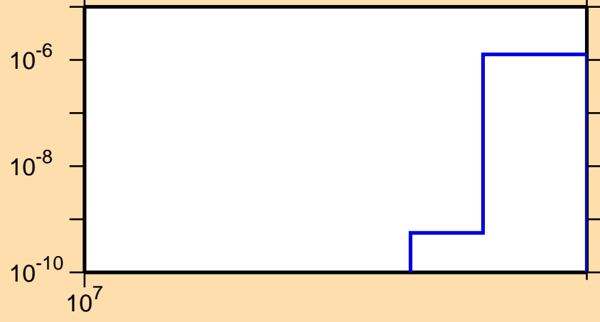
\sigma vs. E for ^{170}\text{Er}(n,\text{nd})
