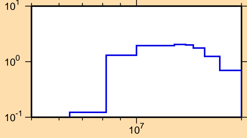
\sigma vs. E for ^{170}\text{Er}(n,2n)
