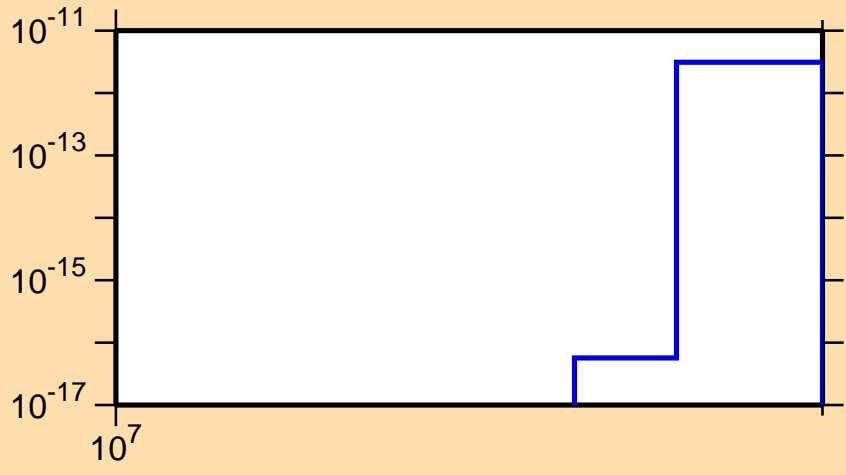
\sigma vs. E for ^{170}\text{Tm}(n,3n\alpha)
