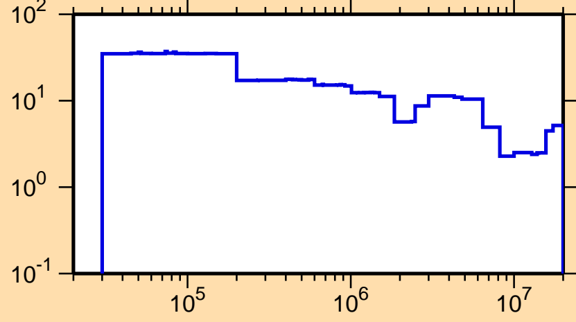
\Delta\sigma/\sigma vs. E for ^{170}\text{Tm}(n,\text{tot.})
