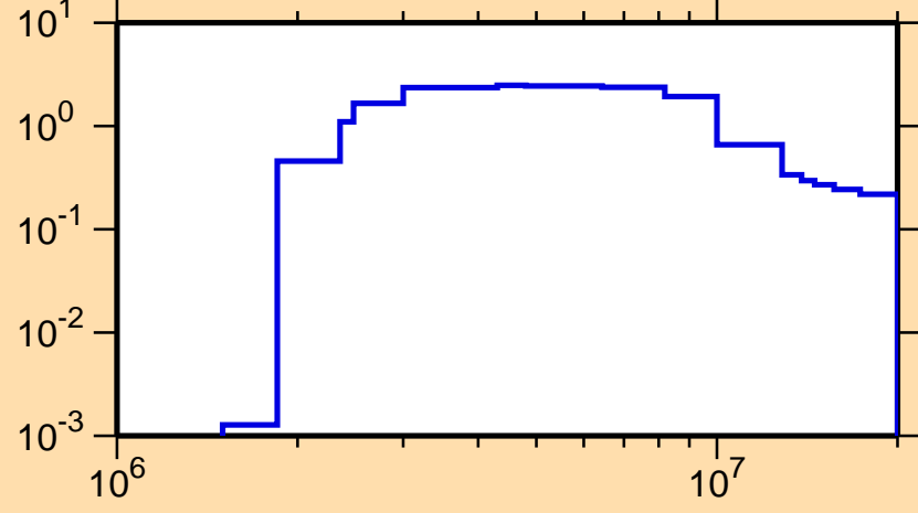
\sigma vs. E for ^{166}\text{Er}(n,n\text{cont.})
