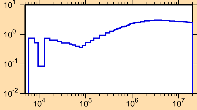
\sigma vs. E for ^{166}\text{Er}(n,\text{nonel.})
