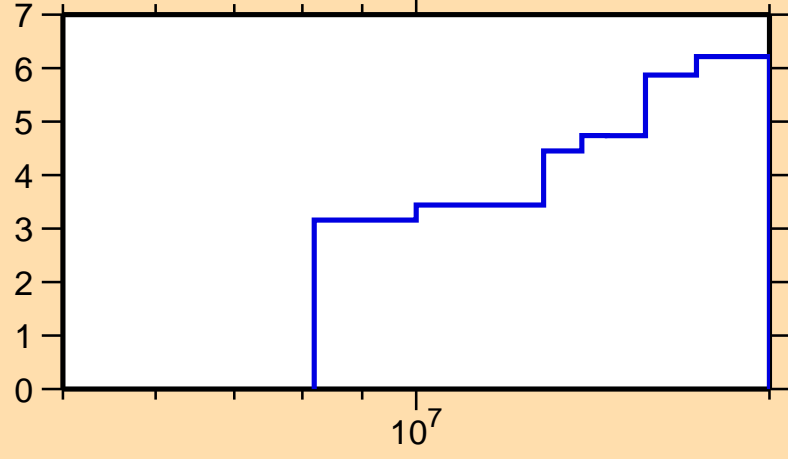
\Delta\sigma/\sigma vs. E for ^{166}\text{Er}(n,\text{tot.})
