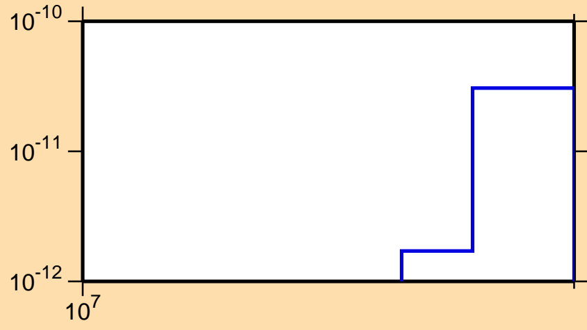
\sigma vs. E for ^{166}\text{Er}(n,p\alpha)
