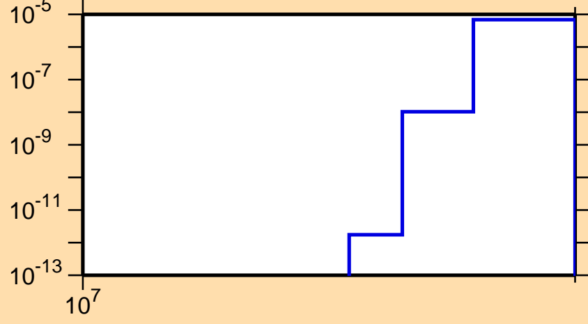
\sigma vs. E for ^{171}\text{Tm}(n,2np)
