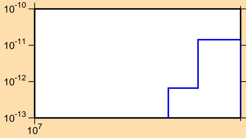
\sigma vs. E for ^{171}\text{Tm}(n,p\alpha)
