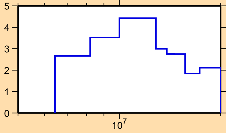
\Delta\sigma/\sigma vs. E for ^{171}\text{Tm}(n,\text{tot.})
