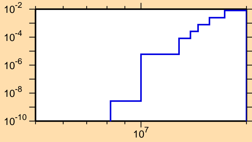
\sigma vs. E for ^{171}\text{Tm}(n,np)
