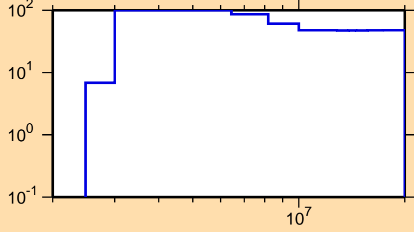
\Delta\sigma/\sigma vs. E for ^{171}\text{Tm}(n,p)
