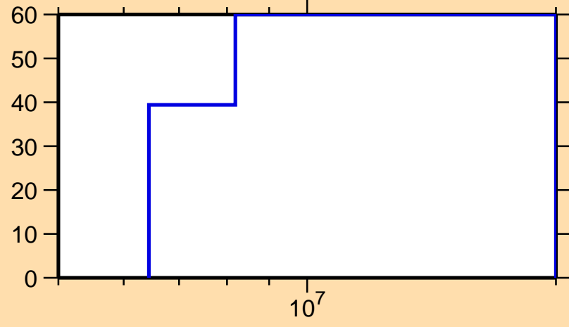
\Delta\sigma/\sigma vs. E for ^{171}\text{Tm}(n,\text{inel.})
