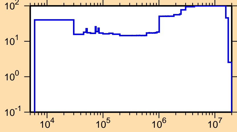
\Delta\sigma/\sigma vs. E for ^{171}\text{Tm}(n,n_1)
