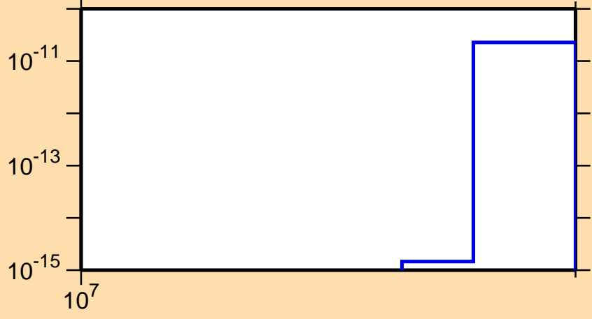
\sigma vs. E for ^{171}\text{Tm}(n,3n\alpha)
