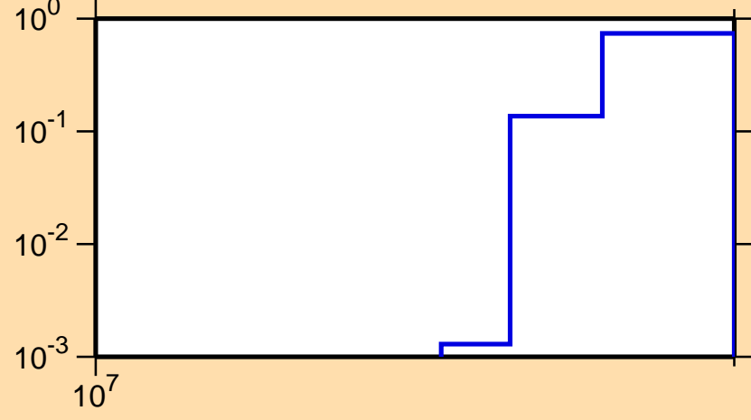
\sigma vs. E for ^{163}\text{Ho}(n,3n)
