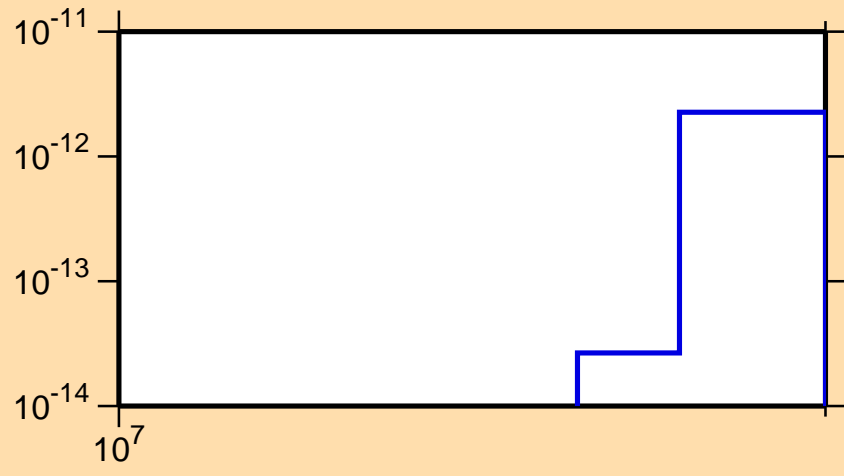
\sigma vs. E for ^{163}\text{Ho} (mt 45)
