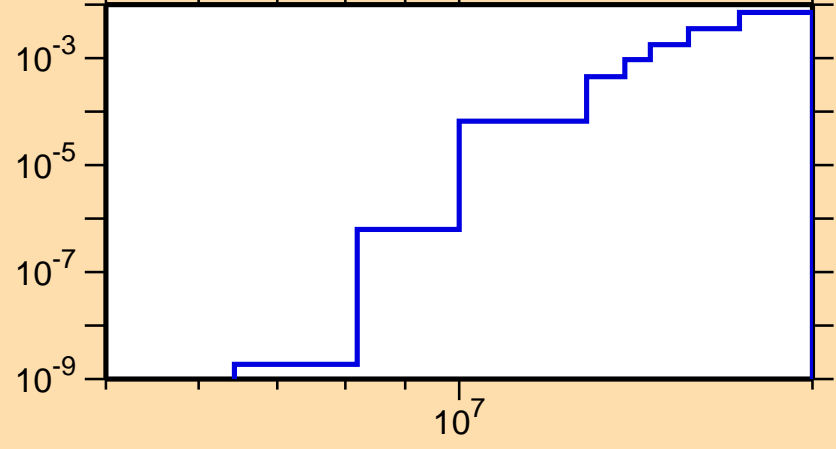
\sigma vs. E for ^{163}\text{Ho}(n,d)
