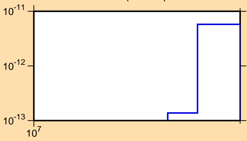
\sigma vs. E for ^{163}\text{Ho} (mt117)
