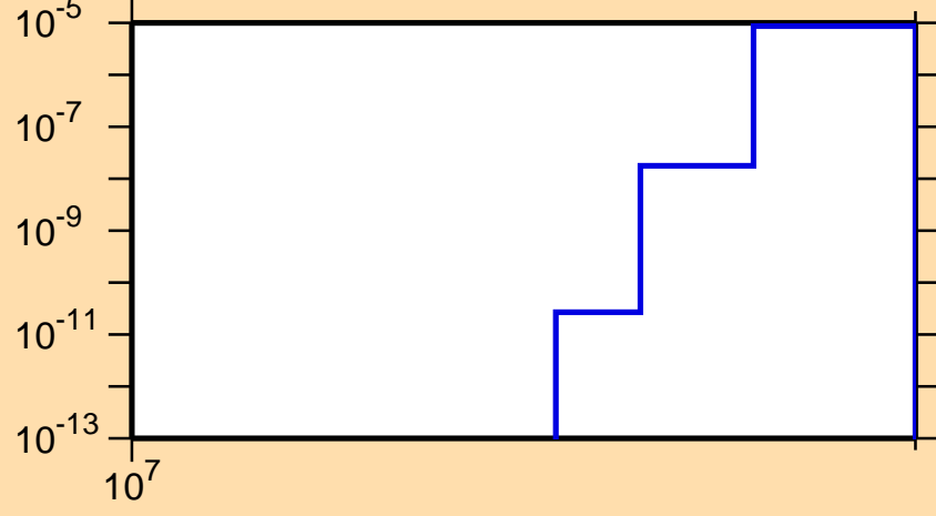
\sigma vs. E for ^{163}\text{Ho}(n,nt)
