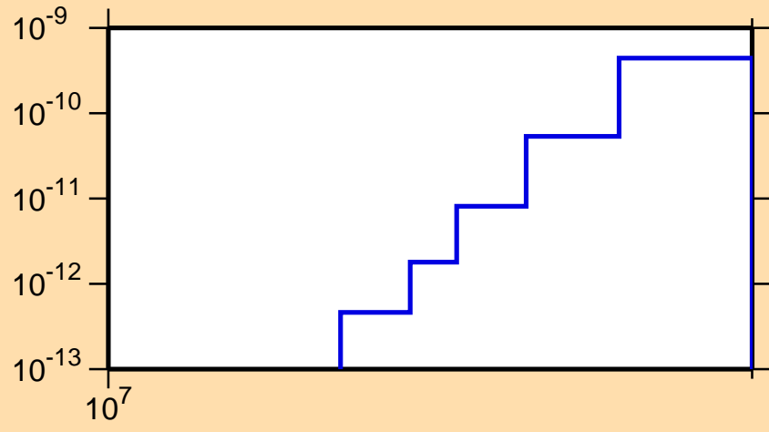
\sigma vs. E for ^{163}\text{Ho}(n,p\alpha)
