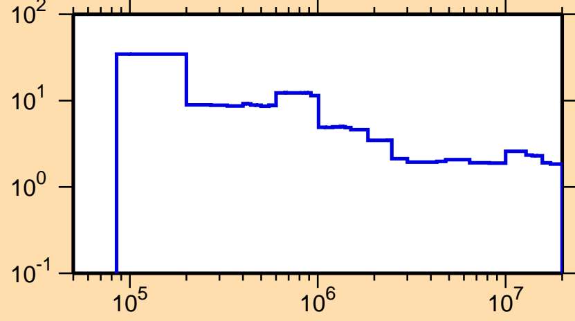
\Delta\sigma/\sigma vs. E for ^{160}\text{Dy}(n,\text{nonel.})
