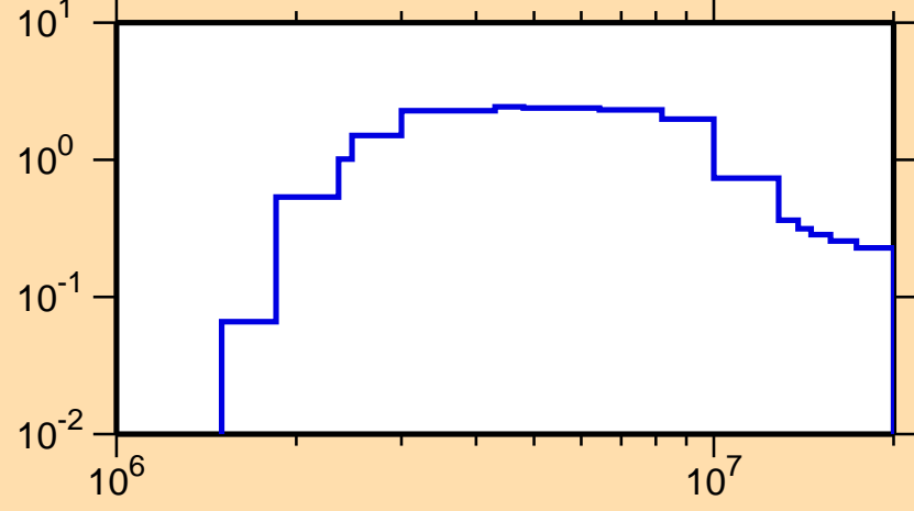
\sigma vs. E for ^{160}\text{Dy}(n,n\text{cont.})
