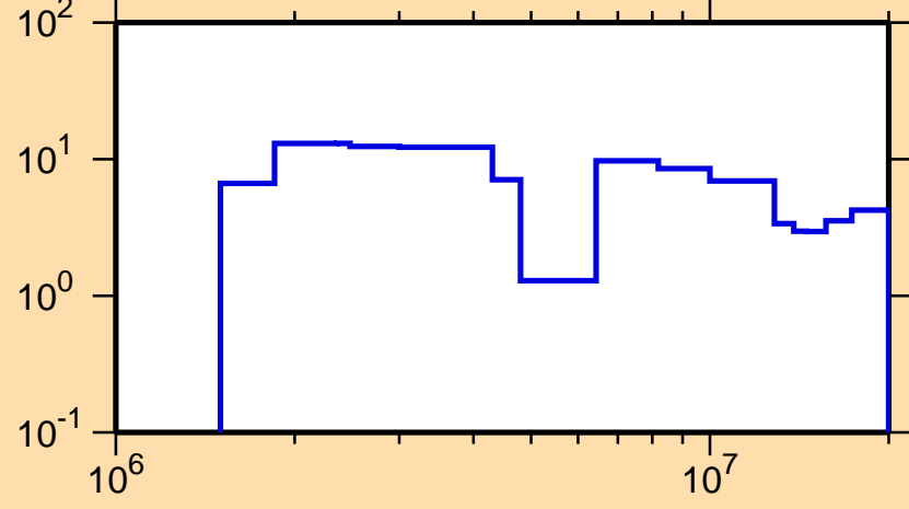
\Delta\sigma/\sigma vs. E for ^{160}\text{Dy}(n,el.)
