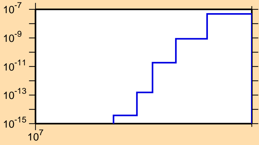
\sigma vs. E for ^{148}\text{Gd}(n,pd)
