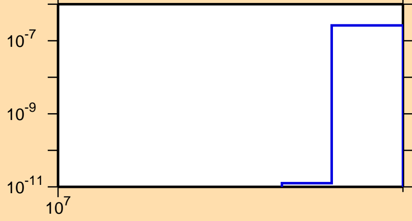
\sigma vs. E for ^{150}\text{Sm}(n,2np)
