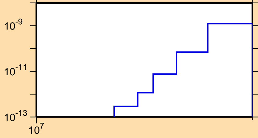
\sigma vs. E for ^{123}\text{Te}(n,p\alpha)
