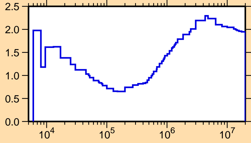
\sigma vs. E for ^{123}\text{Te}(n,\text{nonel.})
