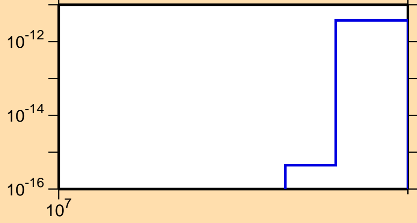
\sigma vs. E for ^{123}\text{Te}(n,pd)
