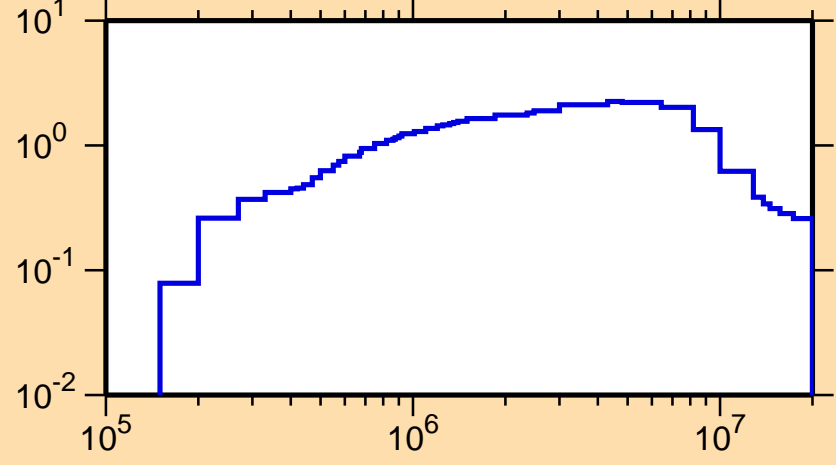
\sigma vs. E for ^{123}\text{Te}(n,\text{inel.})
