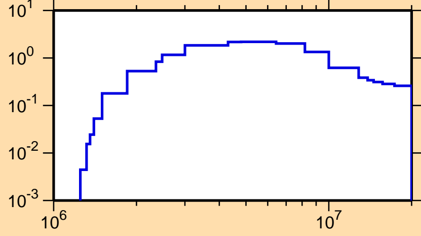
\sigma vs. E for ^{123}\text{Te}(n,n\text{cont.})
