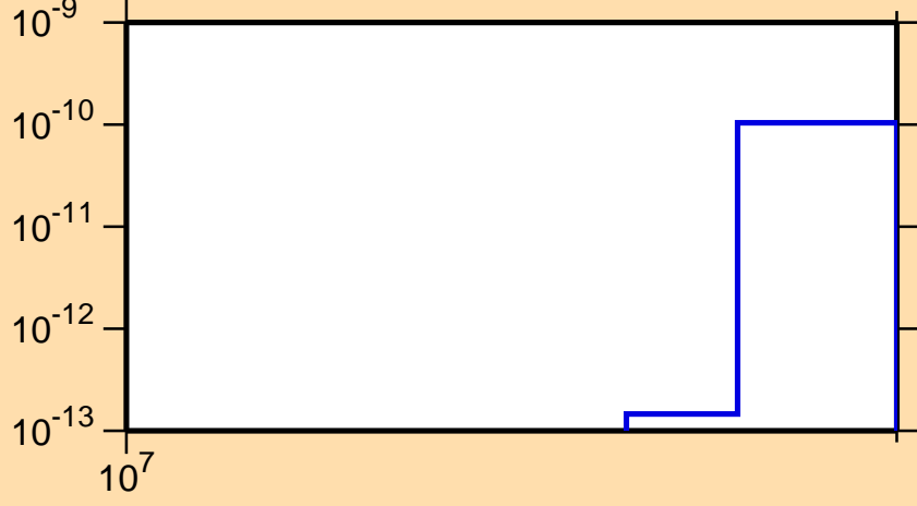
\sigma vs. E for ^{137}\text{Ce}(n,pd)
