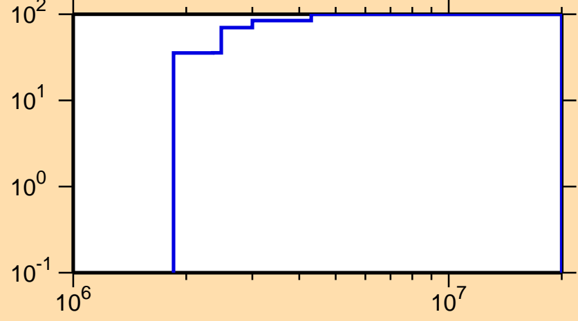
\Delta\sigma/\sigma vs. E for ^{137}\text{Ce}(n,n_1)
