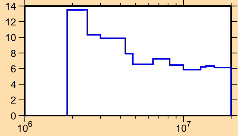
\Delta\sigma/\sigma vs. E for ^{137}\text{Ce}(n,n\text{onel.})
