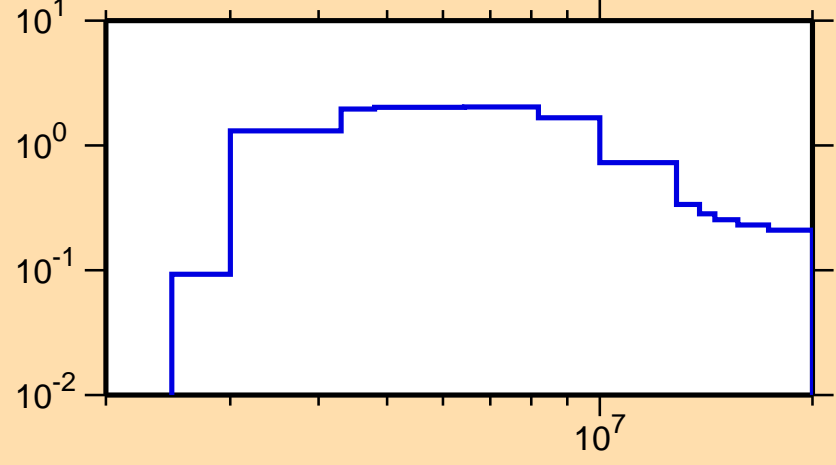
\sigma vs. E for ^{139}\text{Ce}(n,n\text{cont.})
