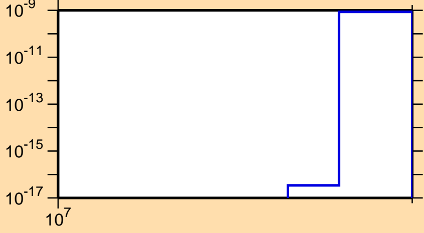
\sigma vs. E for ^{139}\text{Ce}(n,\text{nt})
