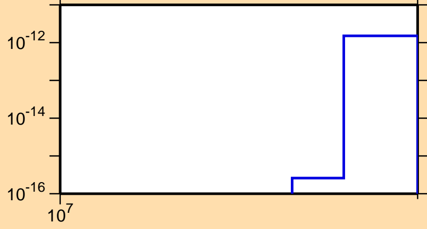
\sigma vs. E for ^{139}\text{Ce}(n,\text{pd})
