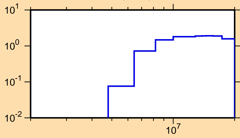
\sigma vs. E for ^{141}\text{Ce}(n,2n)
