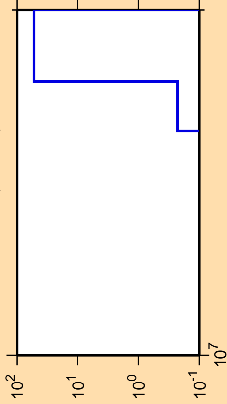
\Delta\sigma/\sigma vs. E for ^{131}\text{Ba}(\text{mt117})
