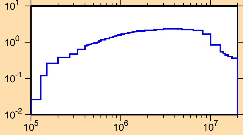
\sigma vs. E for ^{131}\text{Ba}(n,\text{inel.})
