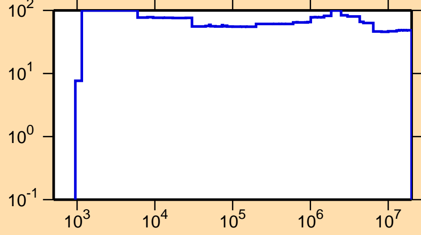
\Delta\sigma/\sigma vs. E for ^{131}\text{Ba}(n,p)
