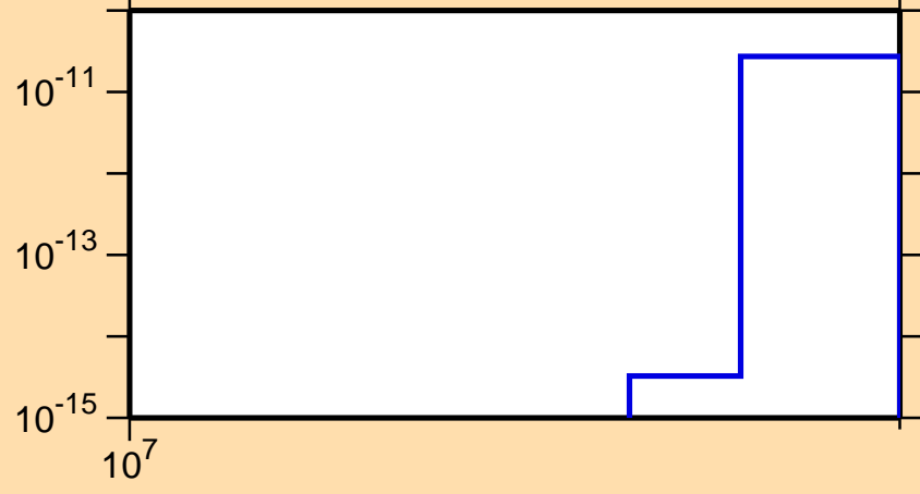
\sigma vs. E for ^{131}\text{Ba} (mt 34)
