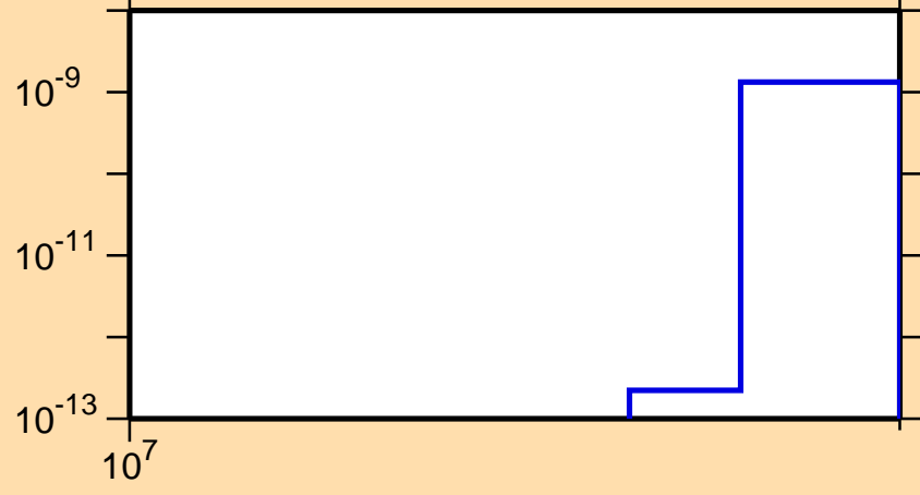
\sigma vs. E for ^{131}\text{Ba}(n,\text{pt})
