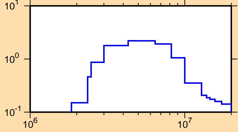
\sigma vs. E for ^{135}\text{Xe}(n,n\text{cont.})
