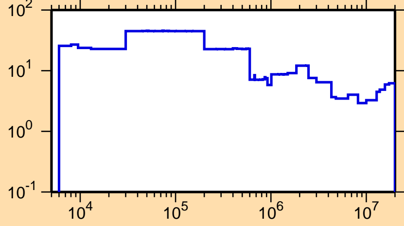
\Delta\sigma/\sigma vs. E for ^{135}\text{Xe}(n,\text{tot.})
