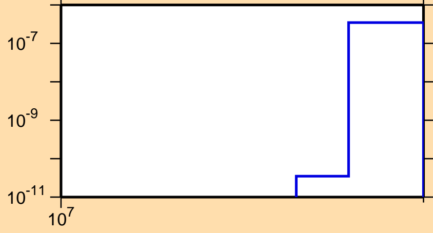
\sigma vs. E for ^{135}\text{Xe}(n,2np)
