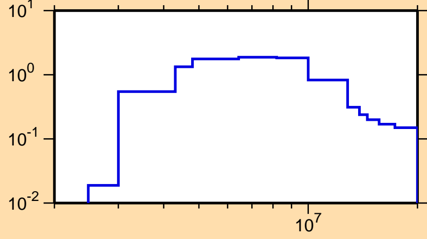
\sigma vs. E for ^{126}\text{Te}(n,n\text{cont.})
