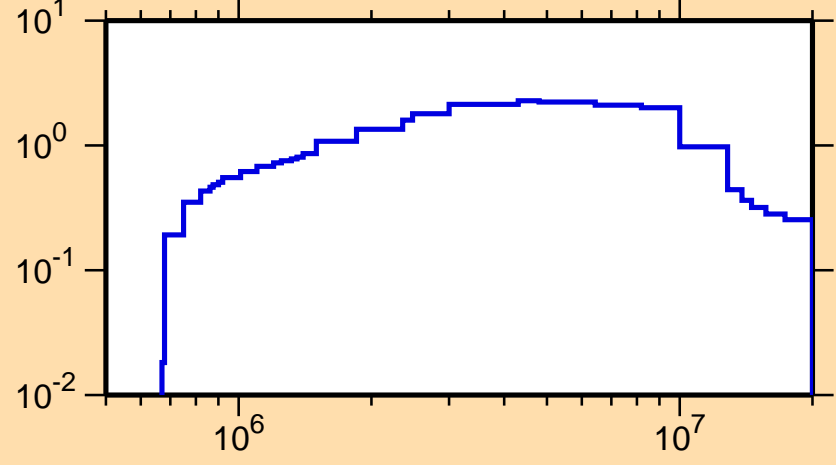
\sigma vs. E for ^{126}\text{Te}(n,\text{inel.})
