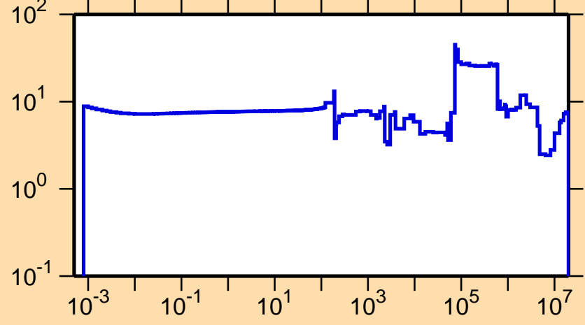
\Delta\sigma/\sigma vs. E for ^{126}\text{Te}(n,\text{tot.})
