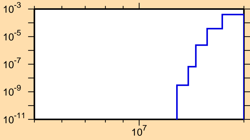
\sigma vs. E for ^{126}\text{Te}(n,t)
