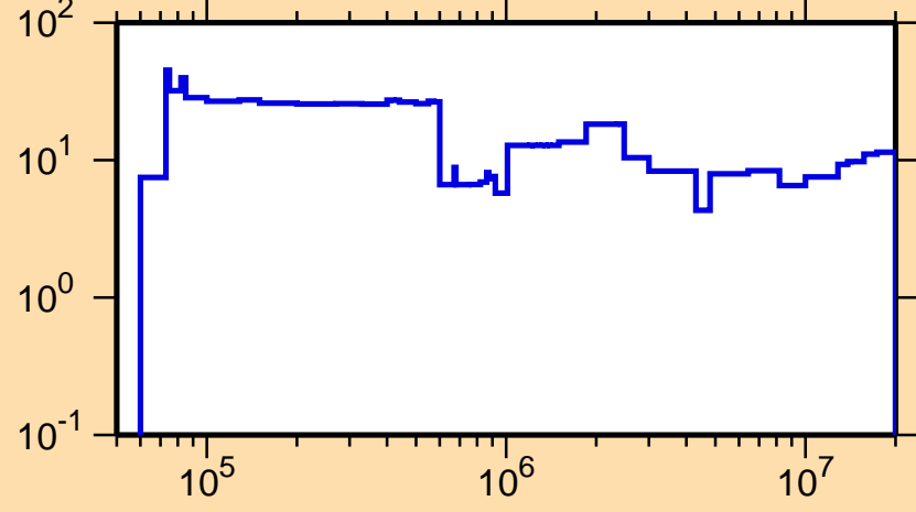
\Delta\sigma/\sigma vs. E for ^{126}\text{Te}(n,\text{el.})
