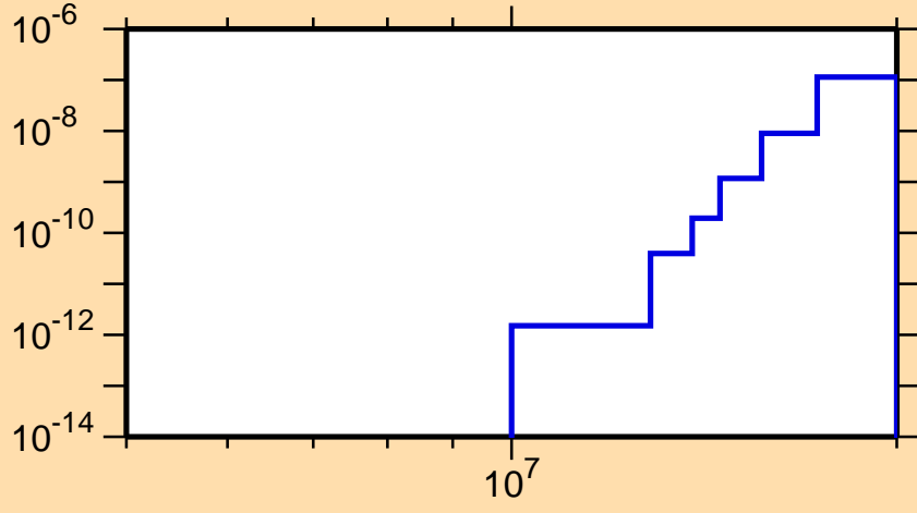
\sigma vs. E for ^{126}\text{Xe}(n,p\alpha)
