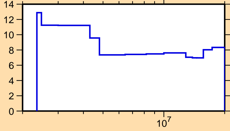
\Delta\sigma/\sigma vs. E for ^{126}\text{Xe}(n,n\text{onel.})
