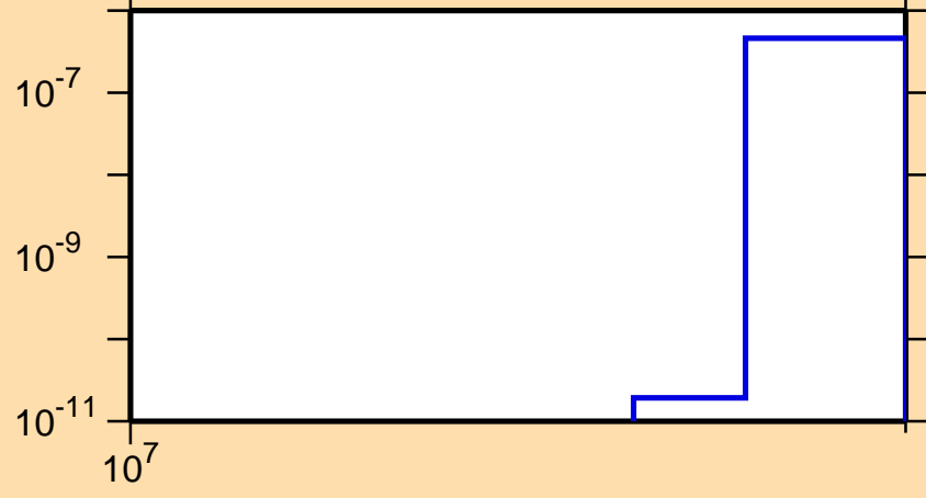
\sigma vs. E for ^{126}\text{Xe}(n,\text{nd})
