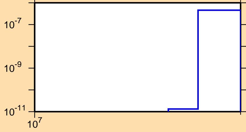
\sigma vs. E for ^{122}\text{Te}(n,nd)
