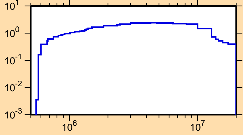
\sigma vs. E for ^{122}\text{Te}(n,\text{inel.})
