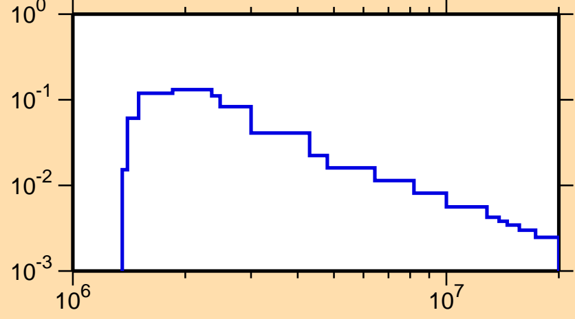
\sigma vs. E for ^{122}\text{Te}(n,n_4)
