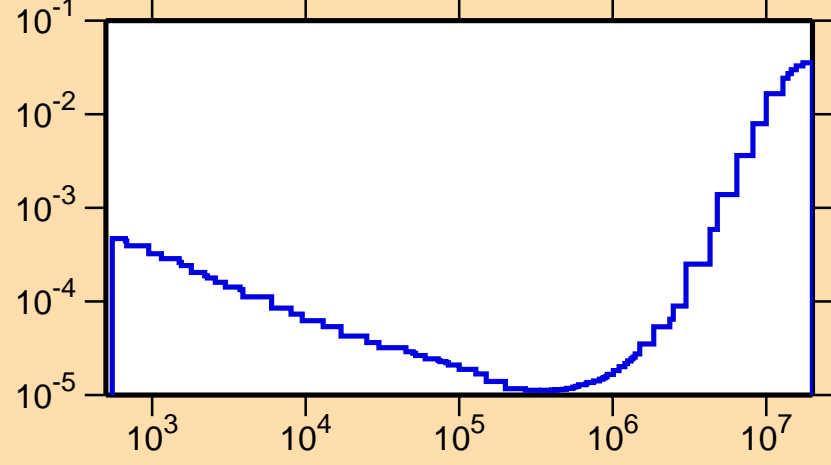
\sigma vs. E for ^{122}\text{Sb}(n,p)
