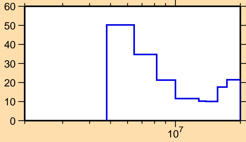
\Delta\sigma/\sigma vs. E for ^{123}\text{Sn}(n,2n)
