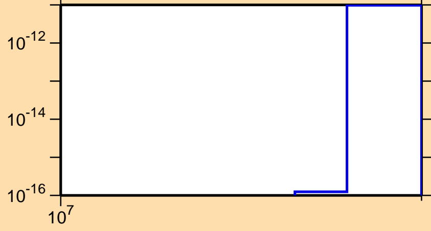
\sigma vs. E for ^{110}\text{Pd}(n,\text{He3})
