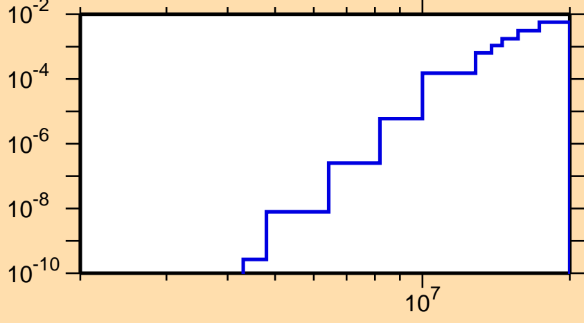
\sigma vs. E for ^{110}\text{Pd}(n,\alpha)
