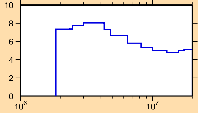
\Delta\sigma/\sigma vs. E for ^{110}\text{Pd}(n,n\text{nonel.})
