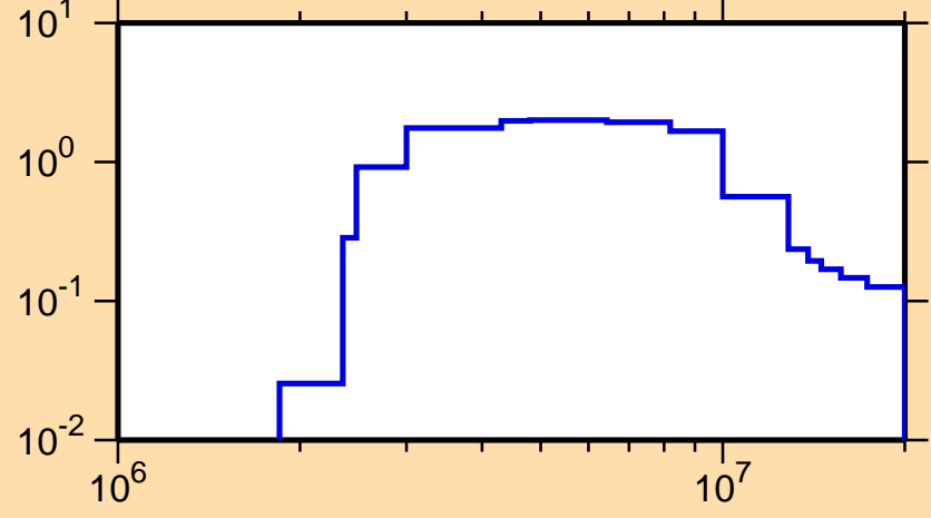
\sigma vs. E for ^{110}\text{Pd}(n,n\text{cont.})
