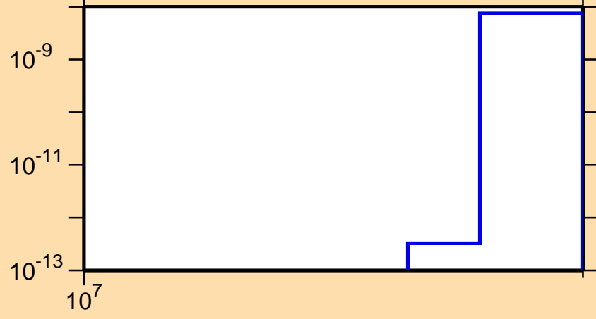
\sigma vs. E for ^{103}\text{Pd}(n,\text{pt})
