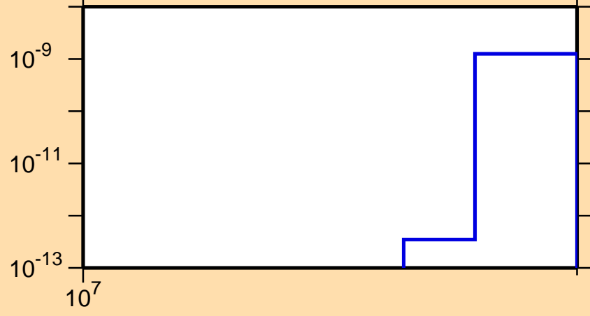
\sigma vs. E for ^{103}\text{Pd}(n,\text{pd})
