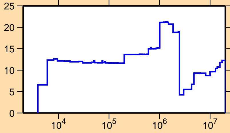
\Delta\sigma/\sigma vs. E for ^{88}\text{Zr}(n,el.)
