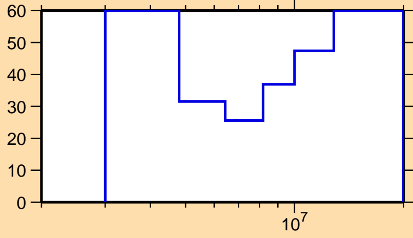
\Delta\sigma/\sigma vs. E for ^{88}\text{Zr}(n,n\text{cont.})
