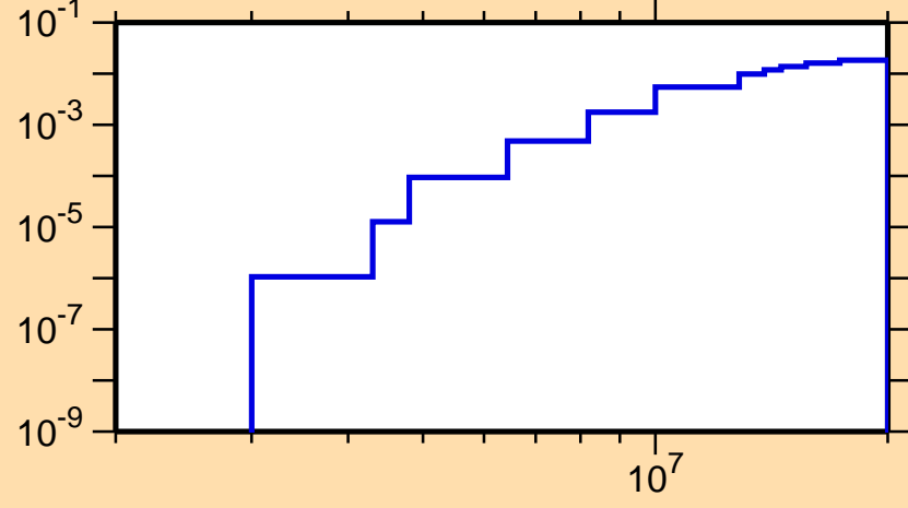
\sigma vs. E for ^{91}\text{Y}(n,p)
