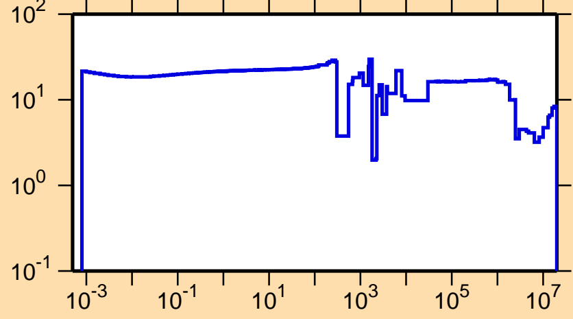
\Delta\sigma/\sigma vs. E for ^{91}\text{Y}(n,\text{tot.})
