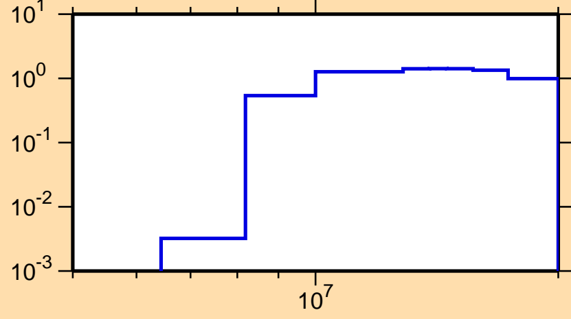
\sigma vs. E for ^{91}\text{Y}(n,2n)
