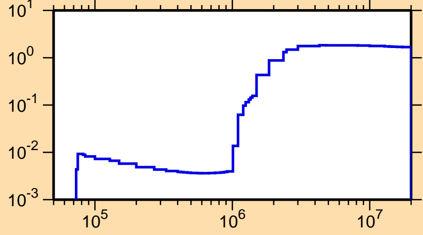
\sigma vs. E for ^{89}\text{Sr}(n,\text{nonel.})
