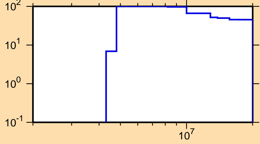
\Delta\sigma/\sigma vs. E for ^{89}\text{Sr}(n,p)
