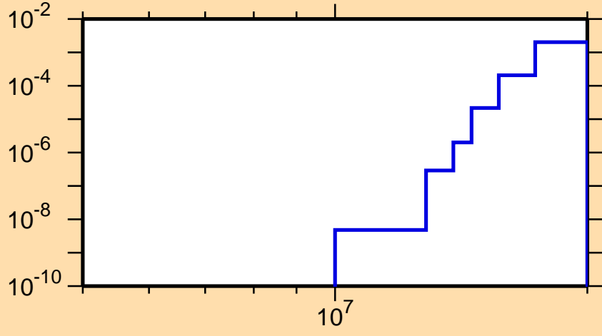
\sigma vs. E for ^{89}\text{Sr}(n,\alpha)
