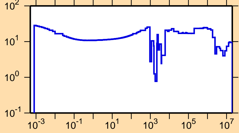
\Delta\sigma/\sigma vs. E for ^{90}\text{Y}(n,\text{tot.})
