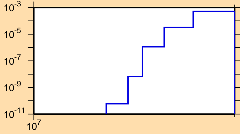
\sigma vs. E for ^{90}\text{Y}(n,\text{nd})
