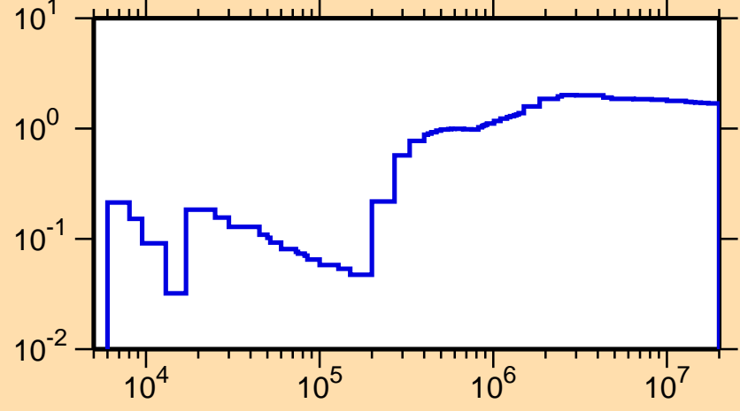
\sigma vs. E for ^{90}\text{Y}(n,\text{nonel.})
