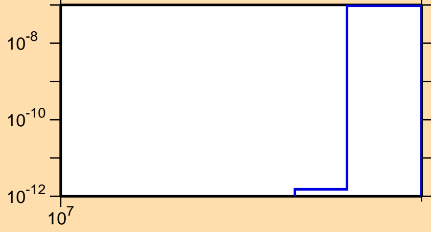
\sigma vs. E for ^{85}\text{Sr}(n,2n\alpha)
