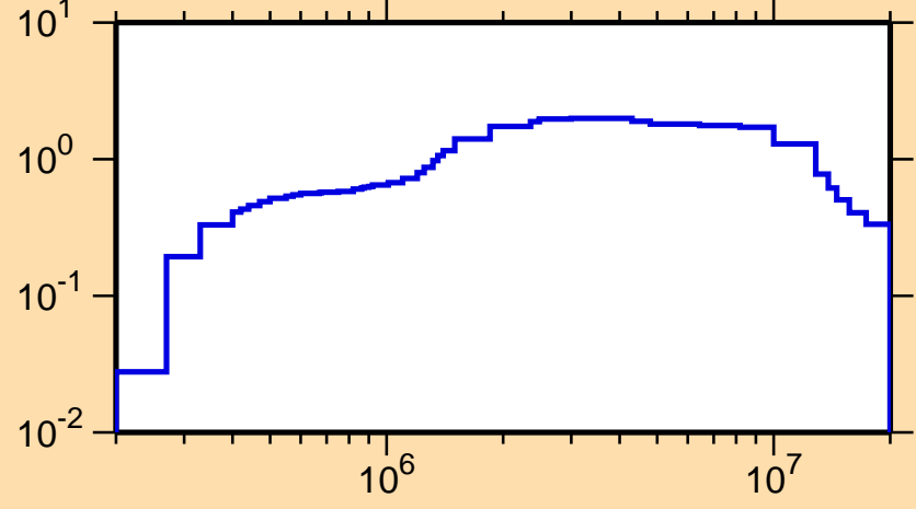
\sigma vs. E for ^{85}\text{Sr}(n,\text{inel.})
