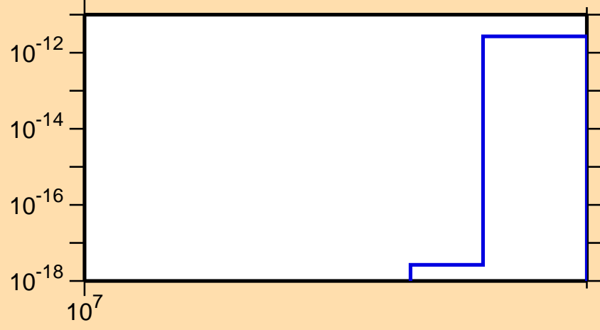
\sigma vs. E for ^{80}\text{Kr}(\text{mt117})
