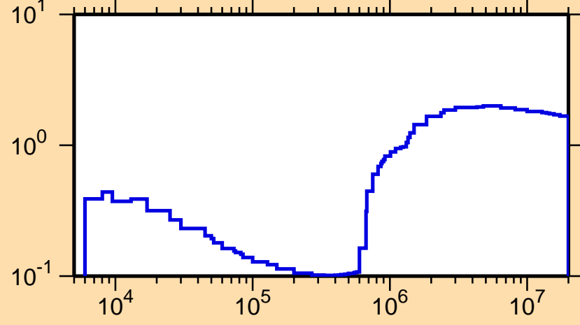
\sigma vs. E for ^{80}\text{Kr}(n,\text{nonel.})
