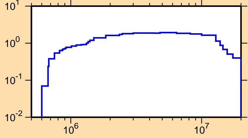
\sigma vs. E for ^{80}\text{Kr}(n,\text{inel.})
