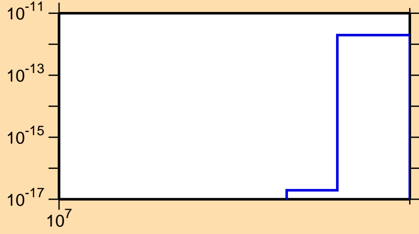
\sigma vs. E for ^{80}\text{Kr}(n,2n\alpha)
