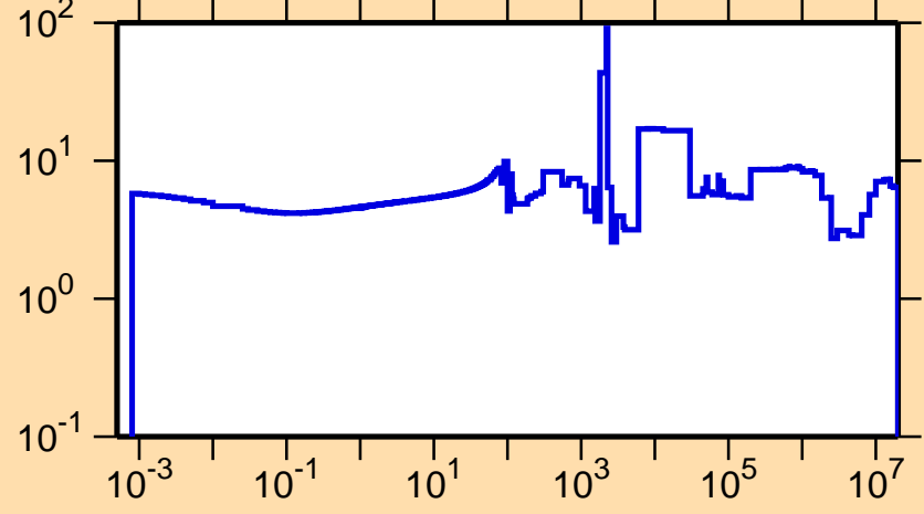
\Delta\sigma/\sigma vs. E for ^{80}\text{Kr}(n,\text{tot.})
