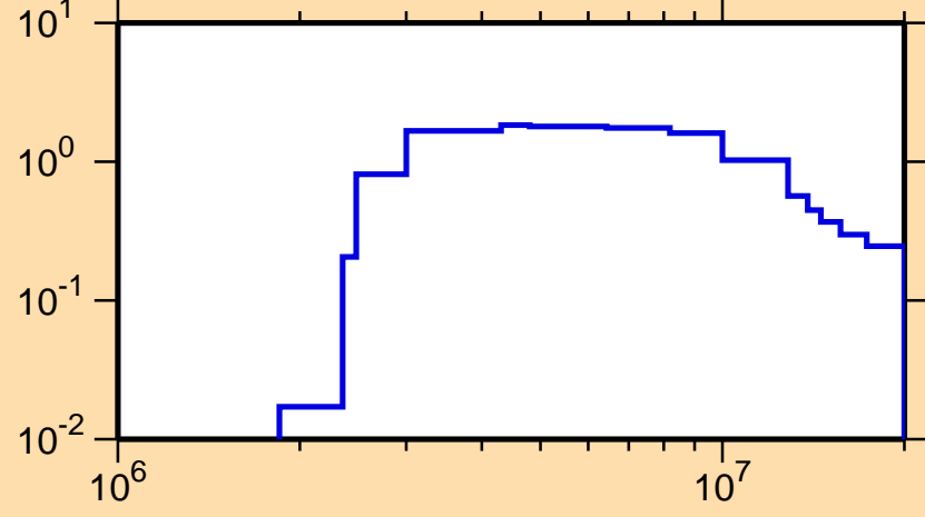
\sigma vs. E for ^{83}\text{Kr}(n,n\text{cont.})
