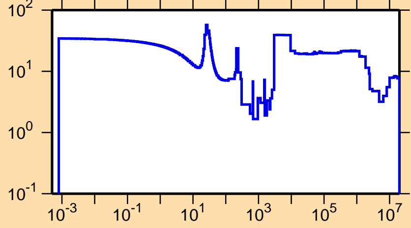
\Delta\sigma/\sigma vs. E for ^{83}\text{Kr}(n,\text{tot.})
