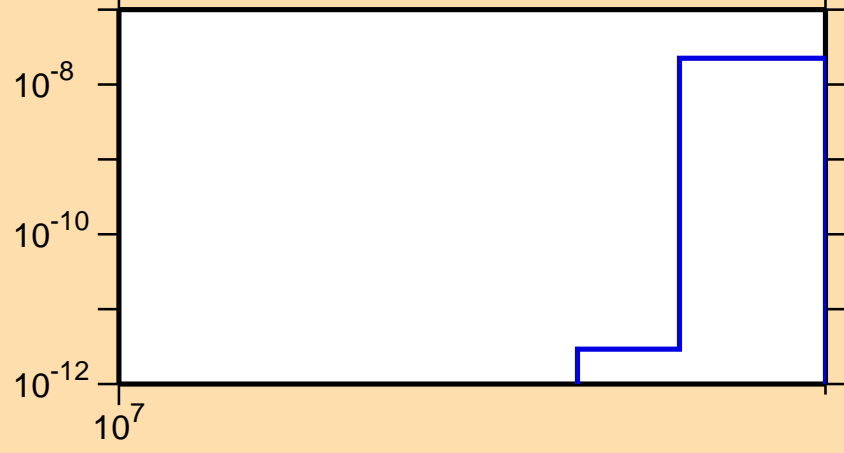
\sigma vs. E for ^{83}\text{Kr}(n,2n\alpha)
