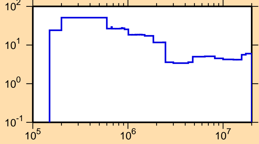
\Delta\sigma/\sigma vs. E for ^{77}\text{As}(n,\text{nonel.})
