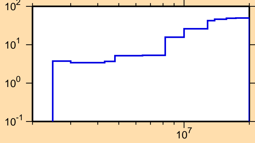
\Delta\sigma/\sigma vs. E for ^{77}\text{As}(n,\text{inel.})
