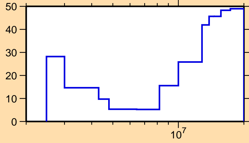
\Delta\sigma/\sigma vs. E for ^{77}\text{As}(n,ncont.)
