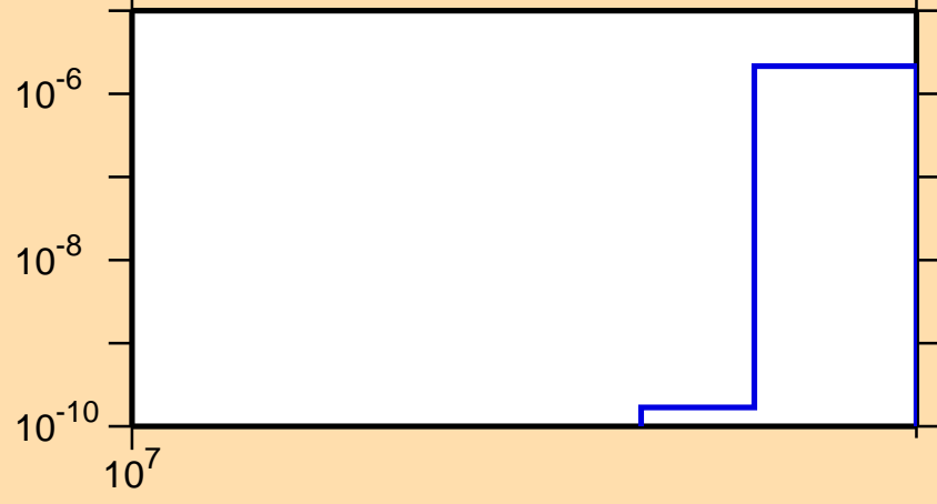
\sigma vs. E for ^{77}\text{As}(n,nt)
