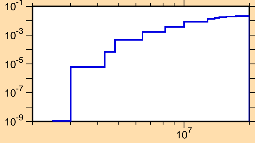
\sigma vs. E for ^{77}\text{As}(n,p)
