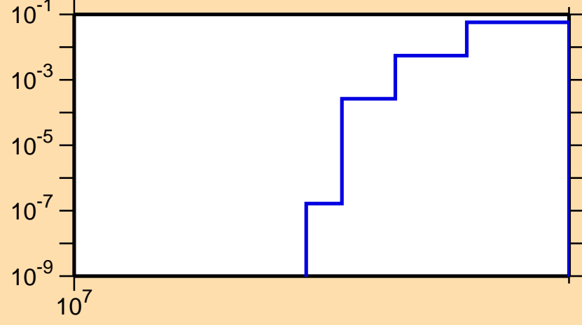
\sigma vs. E for ^{72}\text{As}(n,2np)
