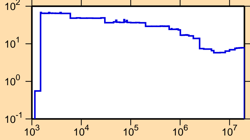
\Delta\sigma/\sigma vs. E for ^{72}\text{As}(n,\text{nonel.})
