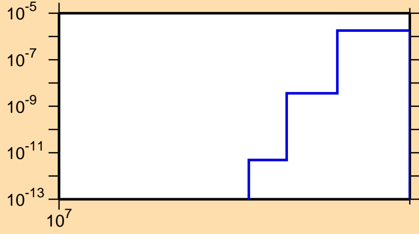
\sigma vs. E for ^{72}\text{As}(n,pd)
