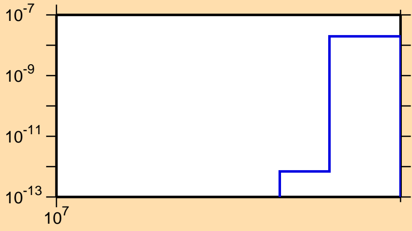
\sigma vs. E for ^{72}\text{As} (mt 34)
