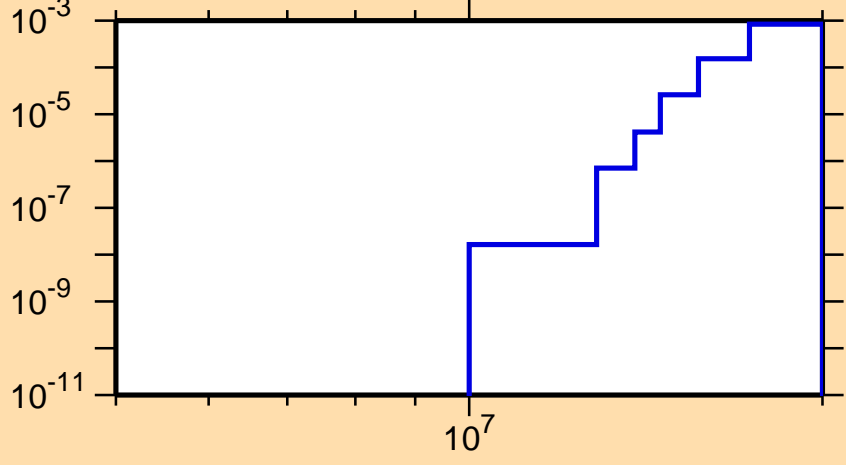
\sigma vs. E for ^{72}\text{As}(n,\text{He3})
