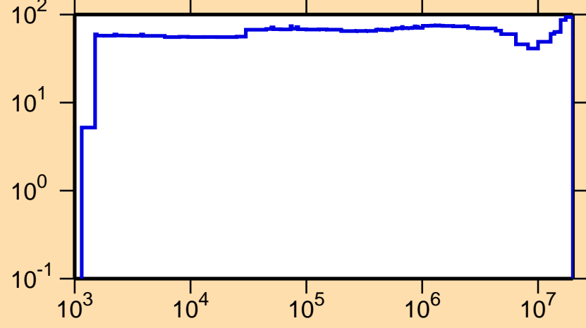
\Delta\sigma/\sigma vs. E for ^{72}\text{As}(n,\gamma)
