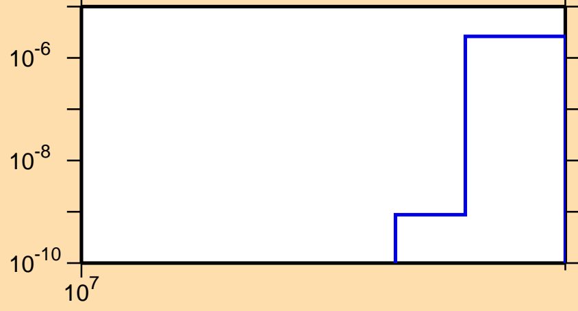
\sigma vs. E for ^{72}\text{As}(n,\text{pt})
