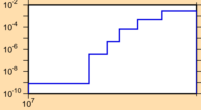
\sigma vs. E for ^{72}\text{As}(n,\text{nd})
