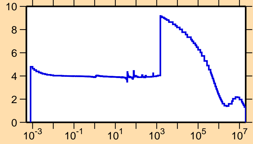
\sigma vs. E for ^{72}\text{As}(n,\text{el.})
