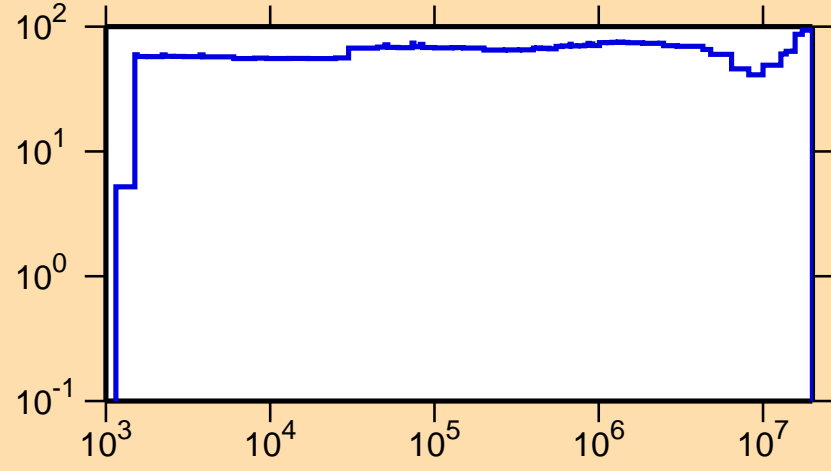
\Delta\sigma/\sigma vs. E for ^{72}\text{As}(n,\gamma)
