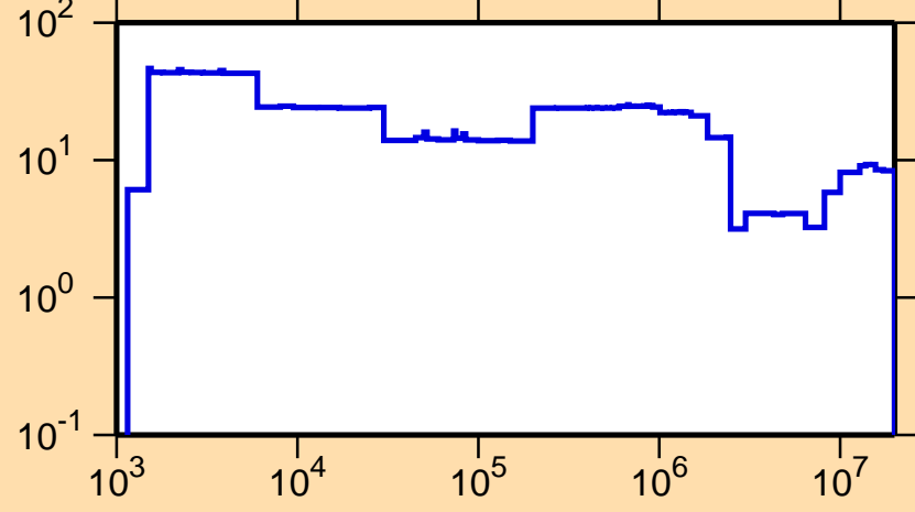
\Delta\sigma/\sigma vs. E for ^{72}\text{As}(n,\text{tot.})
