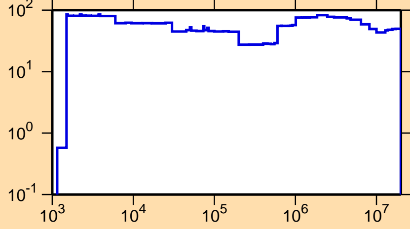
\Delta\sigma/\sigma vs. E for ^{72}\text{As}(n,p)
