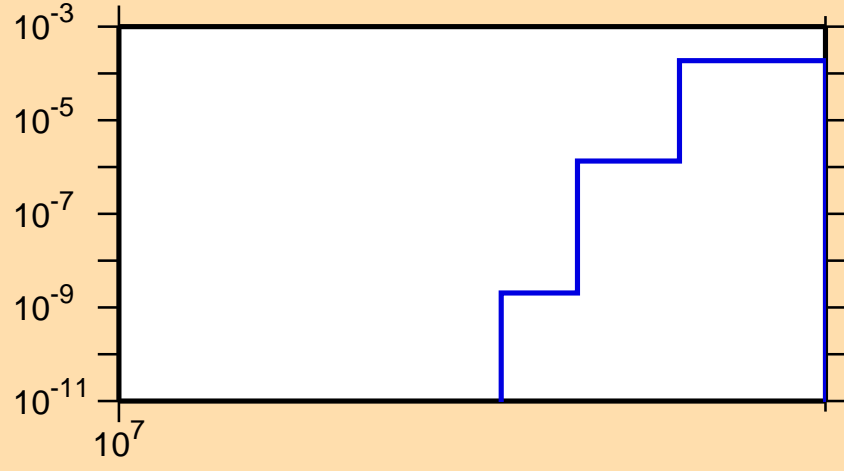
\sigma vs. E for ^{72}\text{As}(n,2n\alpha)
