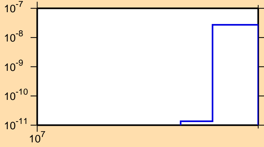
\sigma vs. E for ^{73}\text{As}(n,pd)
