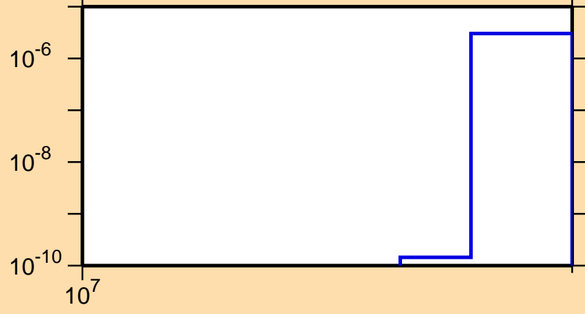
\sigma vs. E for ^{73}\text{As}(n,nt)
