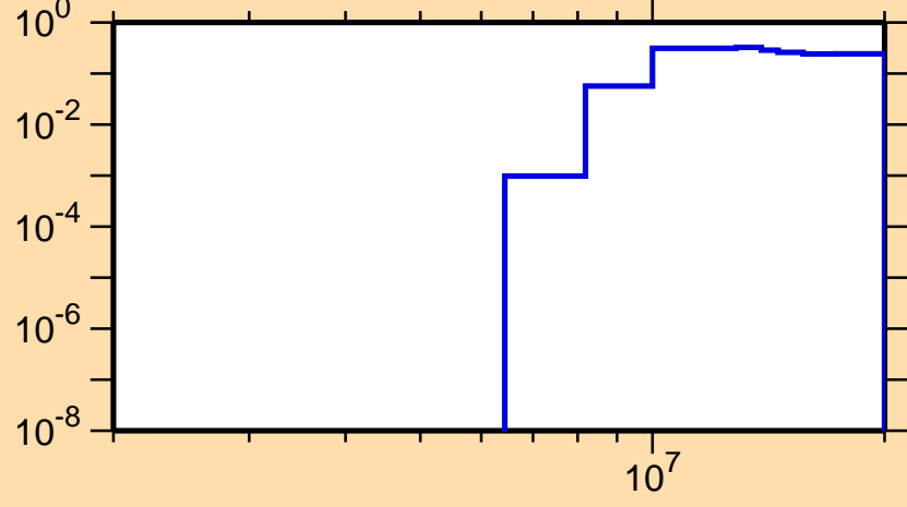
\sigma vs. E for ^{73}\text{As}(n,np)
