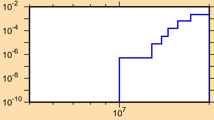
\sigma vs. E for ^{73}\text{As}(n,t)
