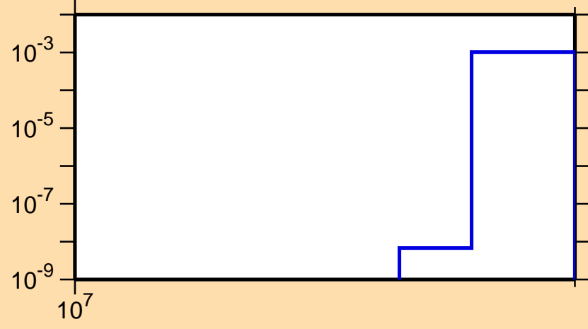
\sigma vs. E for ^{73}\text{As}(n,2np)
