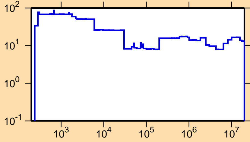
\Delta\sigma/\sigma vs. E for ^{73}\text{As}(n,el.)
