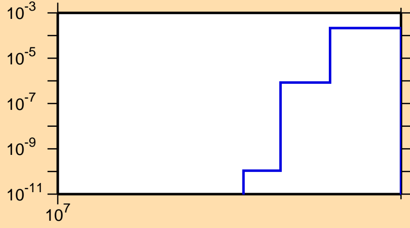
\sigma vs. E for ^{73}\text{As}(n,nd)
