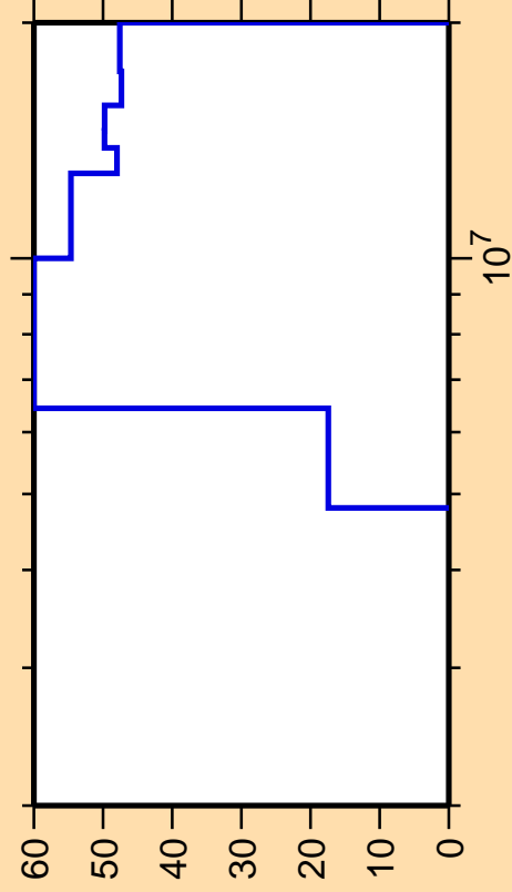
\Delta\sigma/\sigma vs. E for ^{73}\text{As}(n,np)
