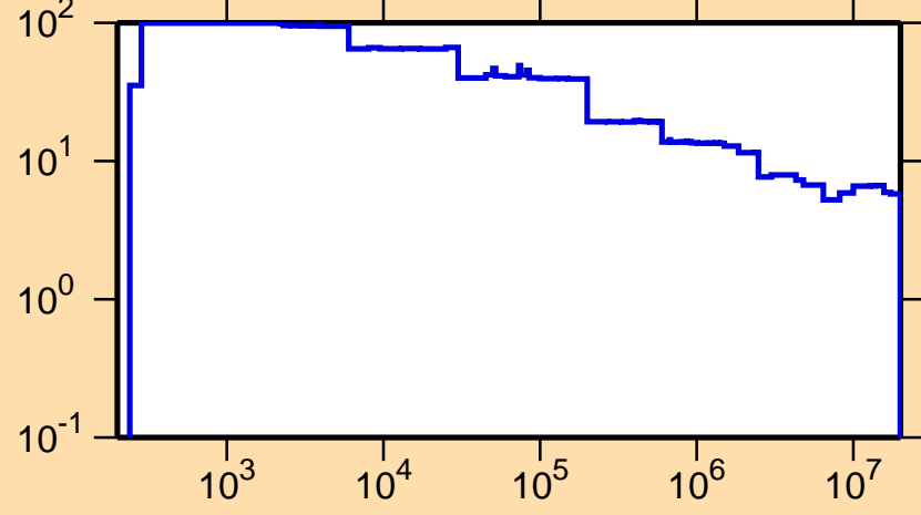
\Delta\sigma/\sigma vs. E for ^{73}\text{As}(n,\text{nonel.})
