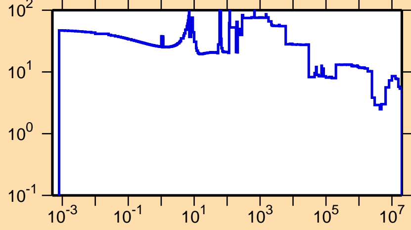
\Delta\sigma/\sigma vs. E for ^{73}\text{As}(n,\text{tot.})
