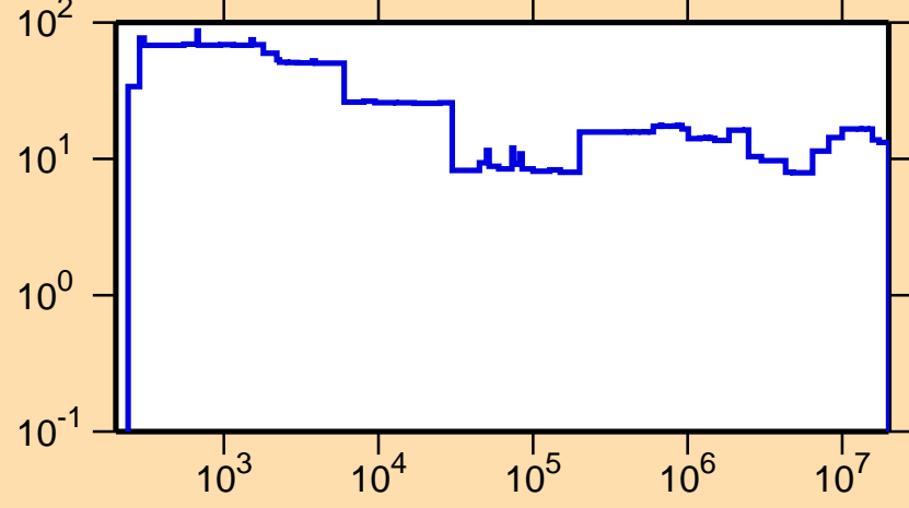
\Delta\sigma/\sigma vs. E for ^{73}\text{As}(n,\text{el.})
