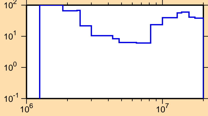
\Delta\sigma/\sigma vs. E for ^{73}\text{As}(n,ncont.)
