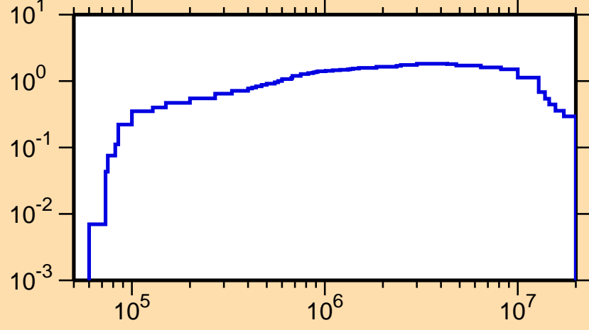
\sigma vs. E for ^{73}\text{As}(n,\text{inel.})
