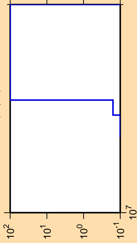
\Delta\sigma/\sigma vs. E for ^{67}\text{Ga}(n,pd)
