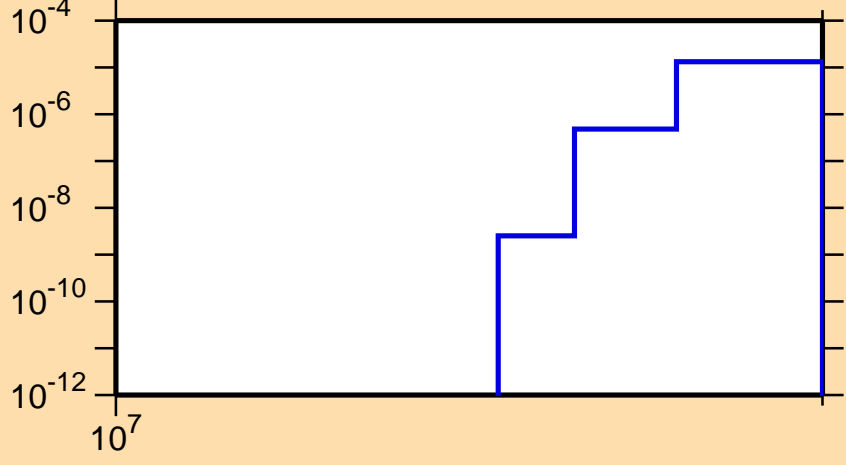
\sigma vs. E for ^{67}\text{Ga}(n,pd)
