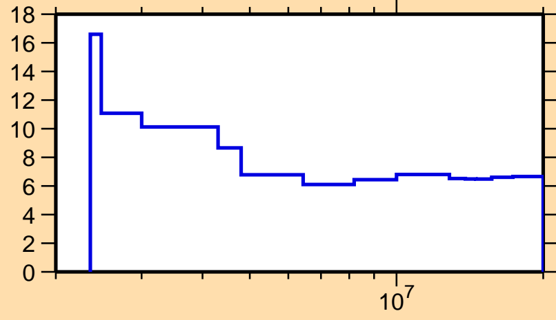
\Delta\sigma/\sigma vs. E for ^{67}\text{Ga}(n,n\text{onel.})
