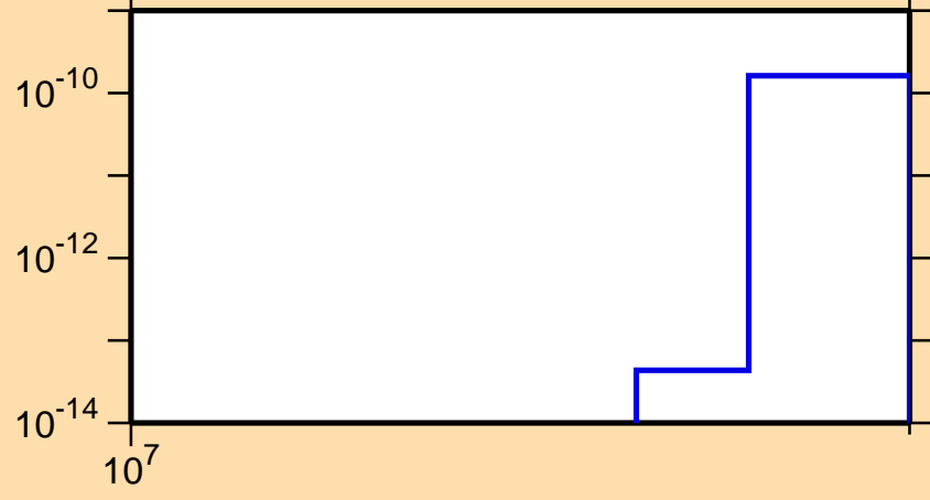
\sigma vs. E for ^{56}\text{Co} (mt 34)
