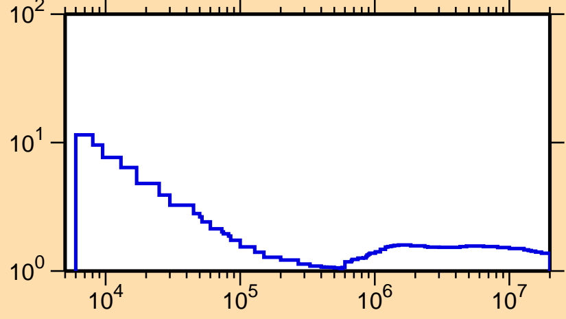
\sigma vs. E for ^{56}\text{Co}(n,\text{nonel.})
