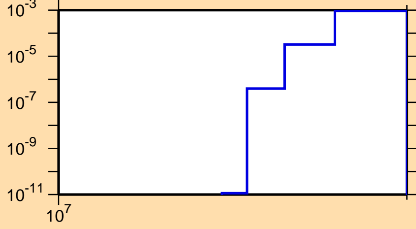
\sigma vs. E for ^{48}\text{V}(n,nd)
