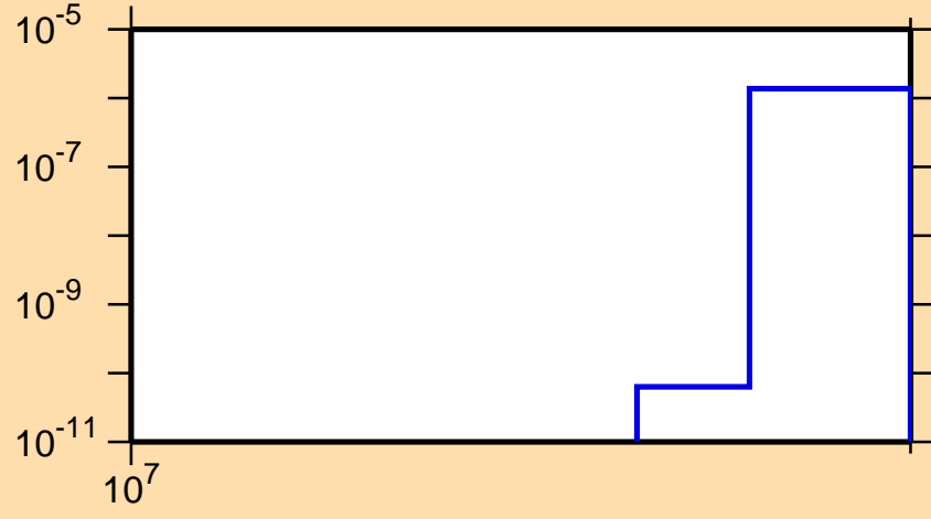
\sigma vs. E for ^{48}\text{V}(n,pd)
