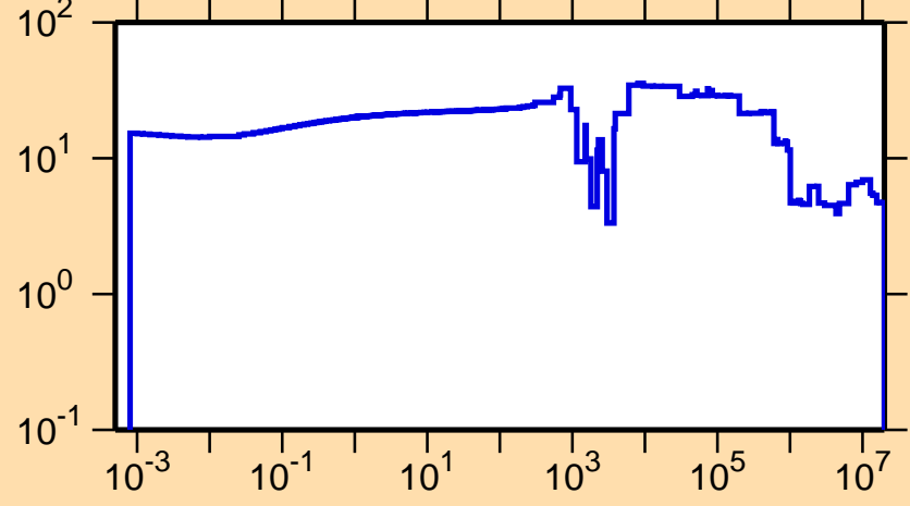
\Delta\sigma/\sigma vs. E for ^{47}\text{Sc}(n,\text{tot.})
