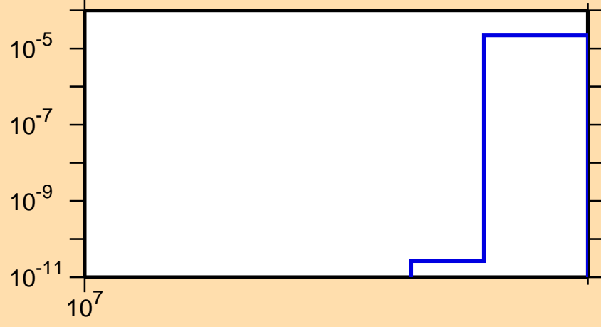
\sigma vs. E for ^{47}\text{Sc}(n,\text{nd})
