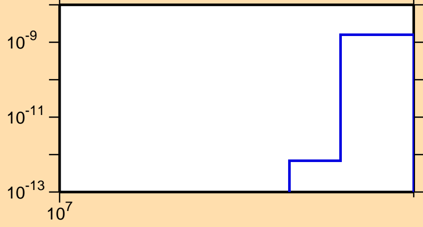
\sigma vs. E for ^{47}\text{Sc}(n,\text{He3})
