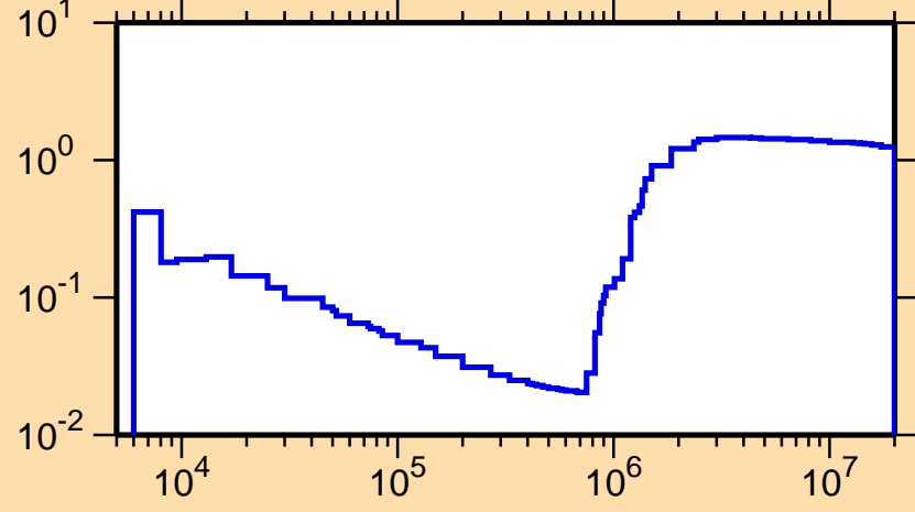
\sigma vs. E for ^{47}\text{Sc}(n,\text{nonel.})
