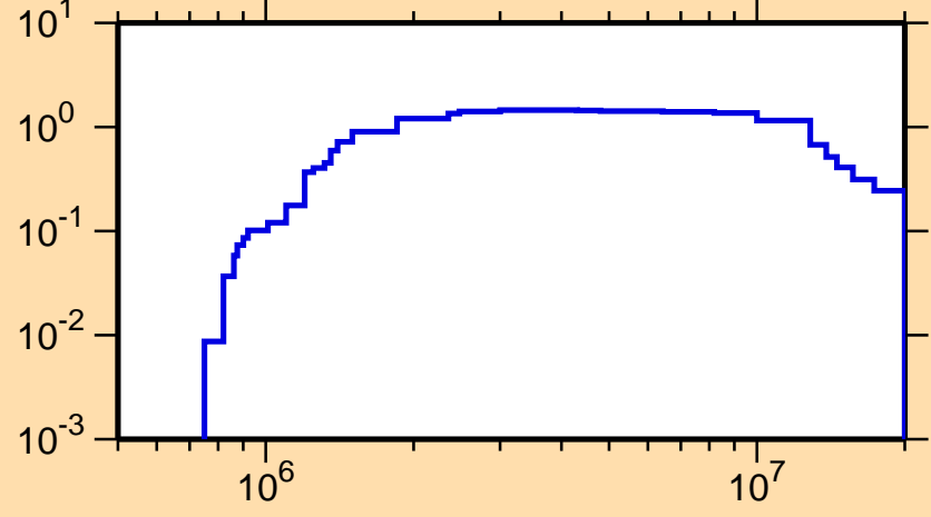
\sigma vs. E for ^{47}\text{Sc}(n,\text{inel.})
