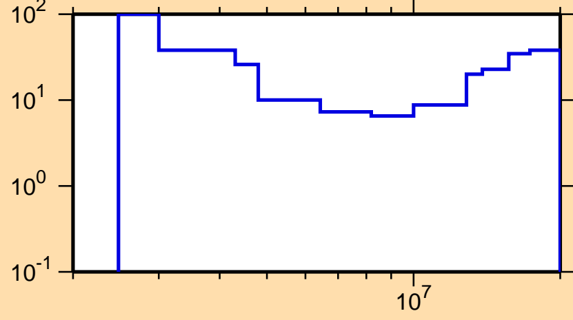
\Delta\sigma/\sigma vs. E for ^{47}\text{Sc}(n,ncont.)
