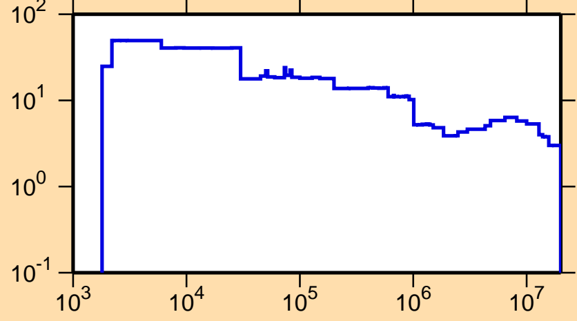
\Delta\sigma/\sigma vs. E for ^{44}\text{Sc}(n,\text{tot.})
