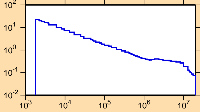
\sigma vs. E for ^{44}\text{Sc}(n,p)
