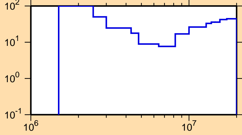
\Delta\sigma/\sigma vs. E for ^{46}\text{Sc}(n,ncont.)
