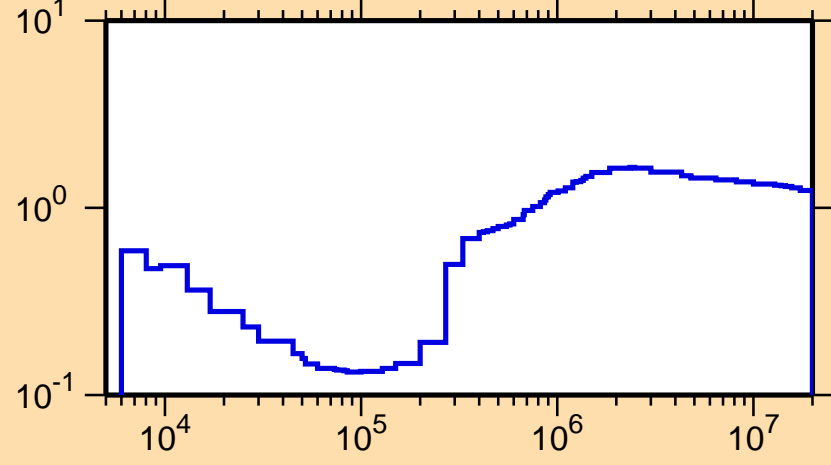
\sigma vs. E for ^{46}\text{Sc}(n,\text{nonel.})
