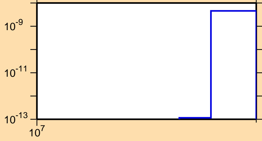
\sigma vs. E for ^{46}\text{Sc}(n,2n\alpha)
