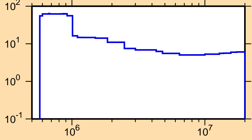
\Delta\sigma/\sigma vs. E for ^{44}\text{Ca}(n,\text{nonel.})
