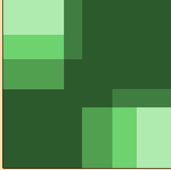
\sigma vs. E for ^{44}\text{Ca}(n,np)
