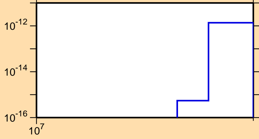
\sigma vs. E for ^{44}\text{Ca}(n,p\alpha)
