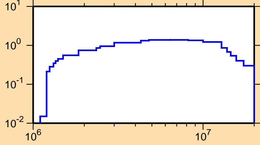
\sigma vs. E for ^{44}\text{Ca}(n,\text{inel.})
