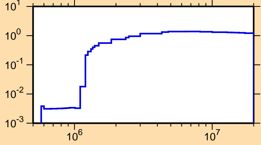
\sigma vs. E for ^{44}\text{Ca}(n,\text{nonel.})
