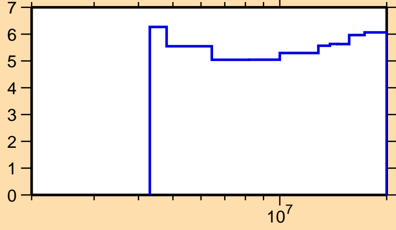
\Delta\sigma/\sigma vs. E for ^{44}\text{Ca}(n,n\text{inel.})
