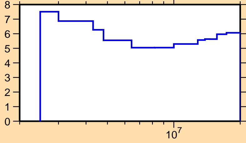
\Delta\sigma/\sigma vs. E for ^{44}\text{Ca}(n,\text{nonel.})
