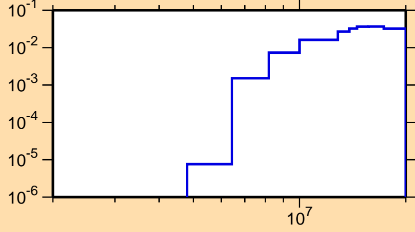
\sigma vs. E for ^{44}\text{Ca}(n,p)
