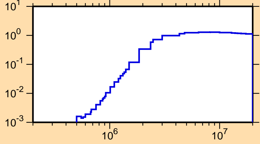
\sigma vs. E for ^{36}\text{Ar}(n,\text{nonel.})
