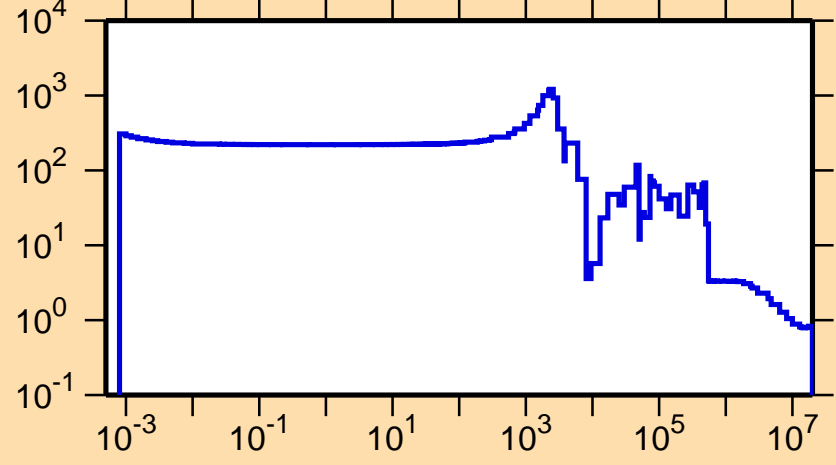
\sigma vs. E for ^{36}\text{Ar}(n,\text{el.})
