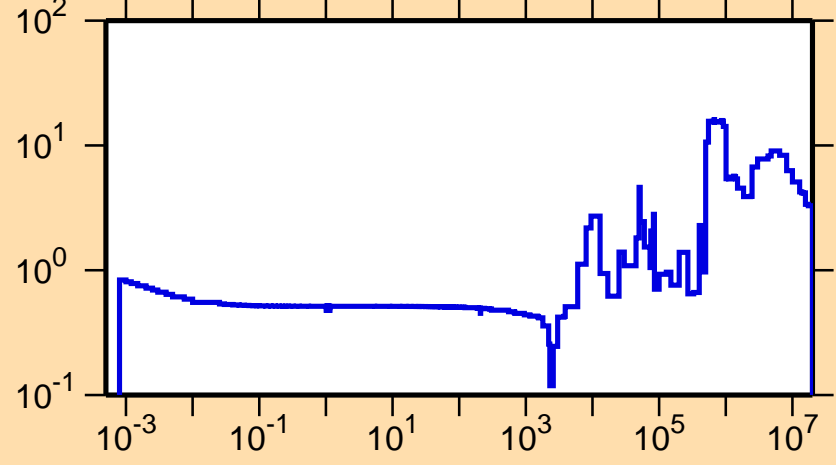
\Delta\sigma/\sigma vs. E for ^{36}\text{Ar}(n,\text{tot.})
