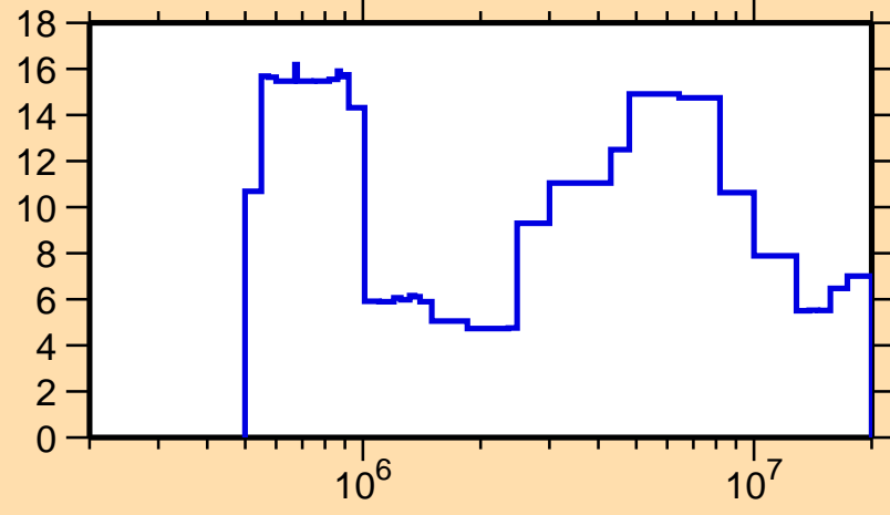
\Delta\sigma/\sigma vs. E for ^{36}\text{Ar}(n,el.)
