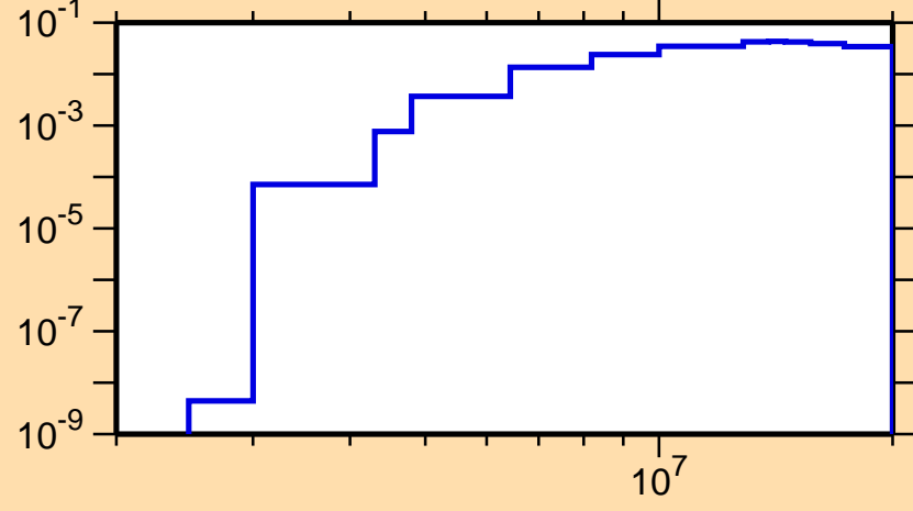
\sigma vs. E for ^{39}\text{Ar}(n,p)
