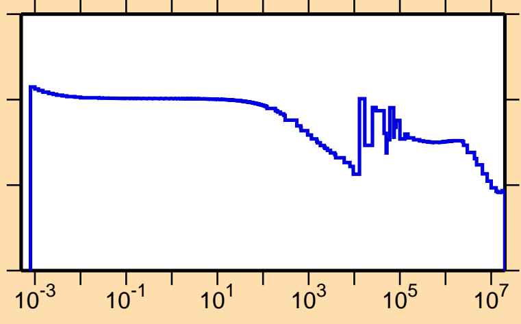
\sigma vs. E for ^{39}\text{Ar}(n,\text{el.})
