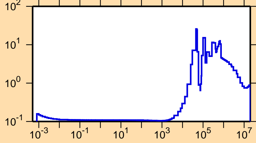
\sigma vs. E for ^{31}\text{Si}(n,\text{el.})
