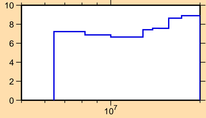
\Delta\sigma/\sigma vs. E for ^{31}\text{Si}(n,n\text{nonel.})
