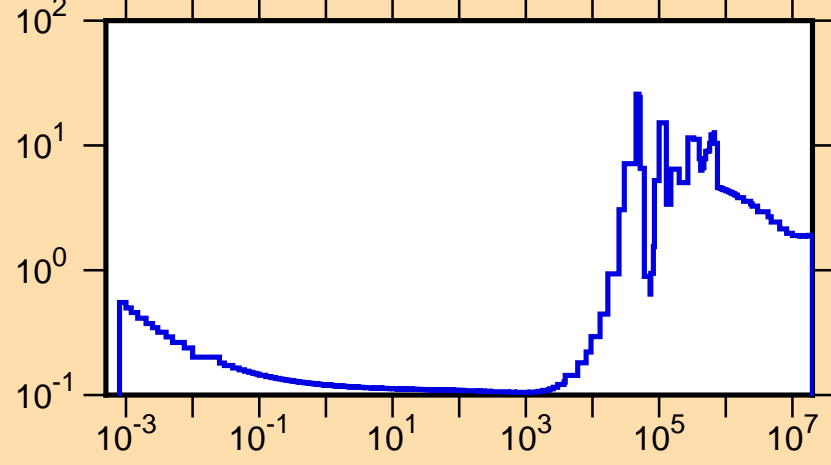
\sigma vs. E for ^{31}\text{Si}(n,\text{tot.})
