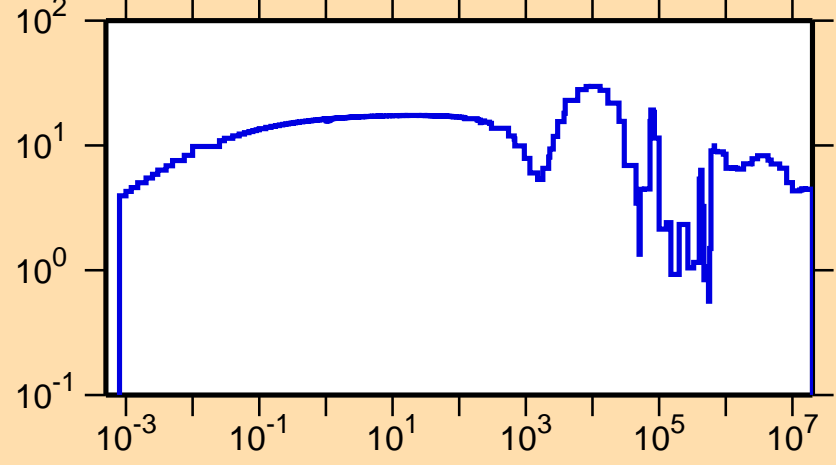
\Delta\sigma/\sigma vs. E for ^{31}\text{Si}(n,\text{tot.})
