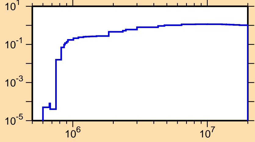
\sigma vs. E for ^{31}\text{Si}(n,\text{nonel.})
