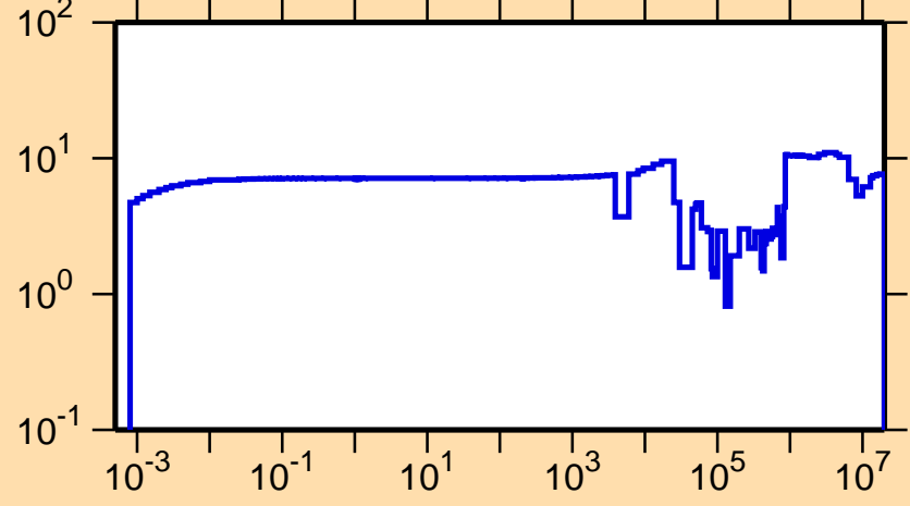
\Delta\sigma/\sigma vs. E for ^{27}\text{Al}(n,\text{el.})
