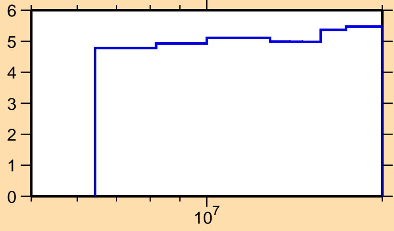
\Delta\sigma/\sigma vs. E for ^{27}\text{Al}(n,n\text{nonel.})
