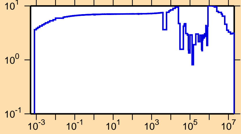
\Delta\sigma/\sigma vs. E for ^{27}\text{Al}(n,\text{tot.})
