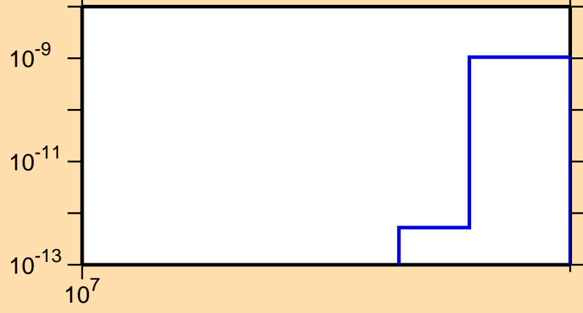
\sigma vs. E for ^{27}\text{Al}(\text{mt117})
