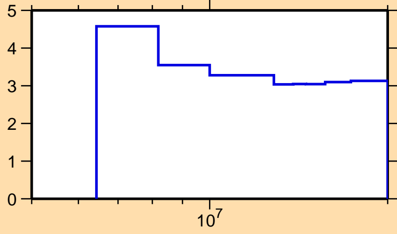
\Delta\sigma/\sigma vs. E for ^{27}\text{Al}(n, tot.)
