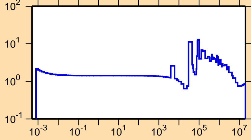
\sigma vs. E for ^{27}\text{Al}(n,\text{el.})
