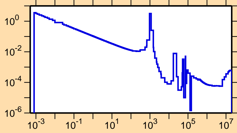
\sigma vs. E for ^{21}\text{Ne}(n,\gamma)
