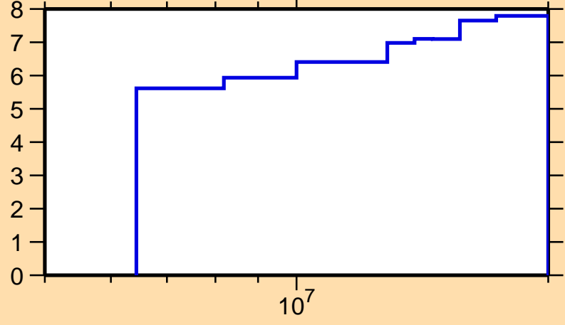
\Delta\sigma/\sigma vs. E for ^{21}\text{Ne}(n,\text{nonel.})
