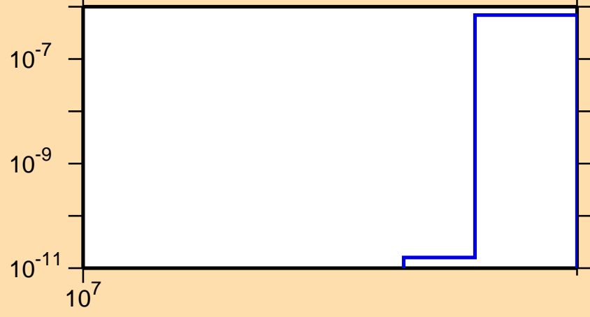
\sigma vs. E for ^{21}\text{Ne}(n,p\alpha)
